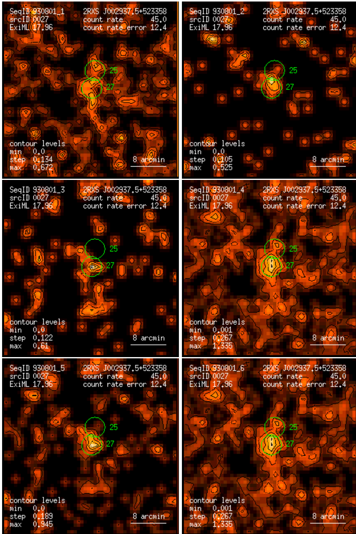
Figure 27: RASS 930801: detection 0027: band rate images, Gaussian filter: (1) PSPC channels 11 – 41, (2) 52 – 90, (3) 91 – 201, (4) 11 – 235, (5) 52 – 201, (6) 11 – 201. Broad band rates in counts/ks. Band rate contour levels in counts/ks/arcmin 2 .
