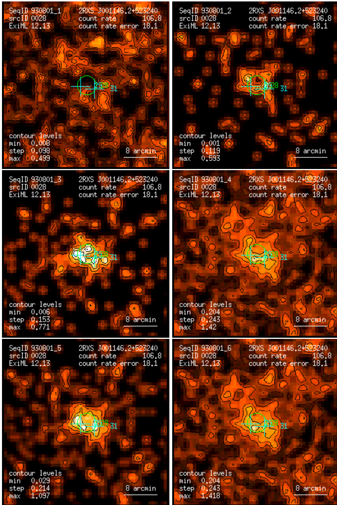
Figure 28: RASS 930801: detection 0028: band rate images, Gaussian filter: (1) PSPC channels 11 – 41, (2) 52 – 90, (3) 91 – 201, (4) 11 – 235, (5) 52 – 201, (6) 11 – 201. Broad band rates in counts/ks. Band rate contour levels in counts/ks/arcmin 2 .
