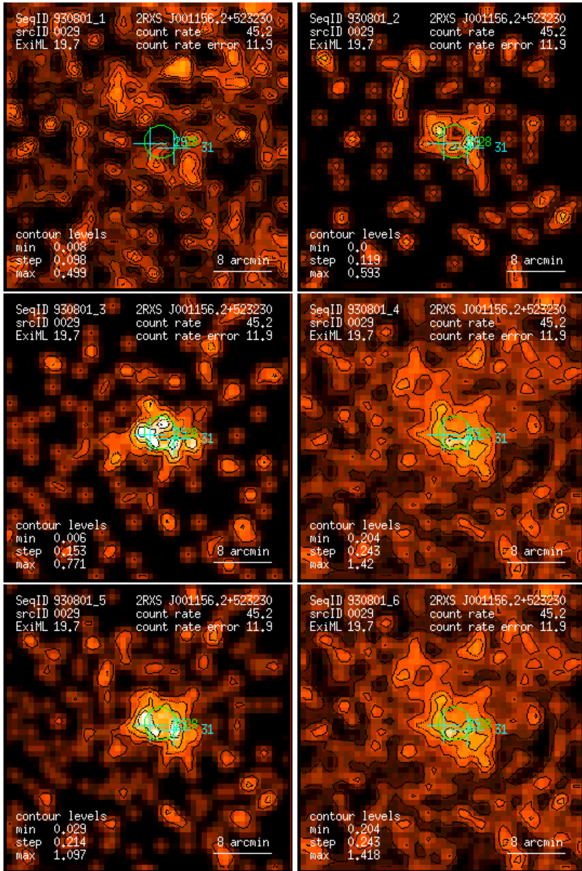
Figure 29: RASS 930801: detection 0029: band rate images, Gaussian filter: (1) PSPC channels 11 – 41, (2) 52 – 90, (3) 91 – 201, (4) 11 – 235, (5) 52 – 201, (6) 11 – 201. Broad band rates in counts/ks. Band rate contour levels in counts/ks/arcmin 2 .
