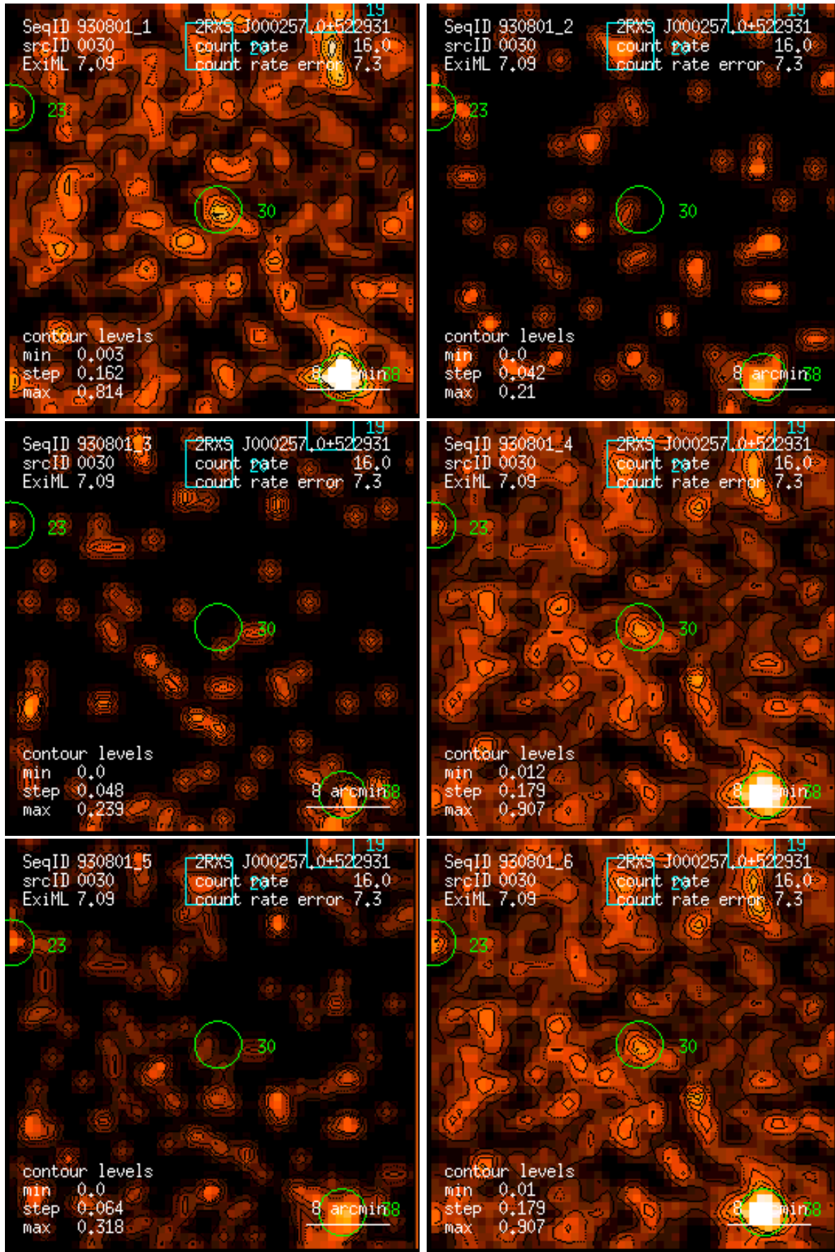
Figure 30: RASS 930801: detection 0030: band rate images, Gaussian filter: (1) PSPC channels 11 – 41, (2) 52 – 90, (3) 91 – 201, (4) 11 – 235, (5) 52 – 201, (6) 11 – 201. Broad band rates in counts/ks. Band rate contour levels in counts/ks/arcmin 2 .
