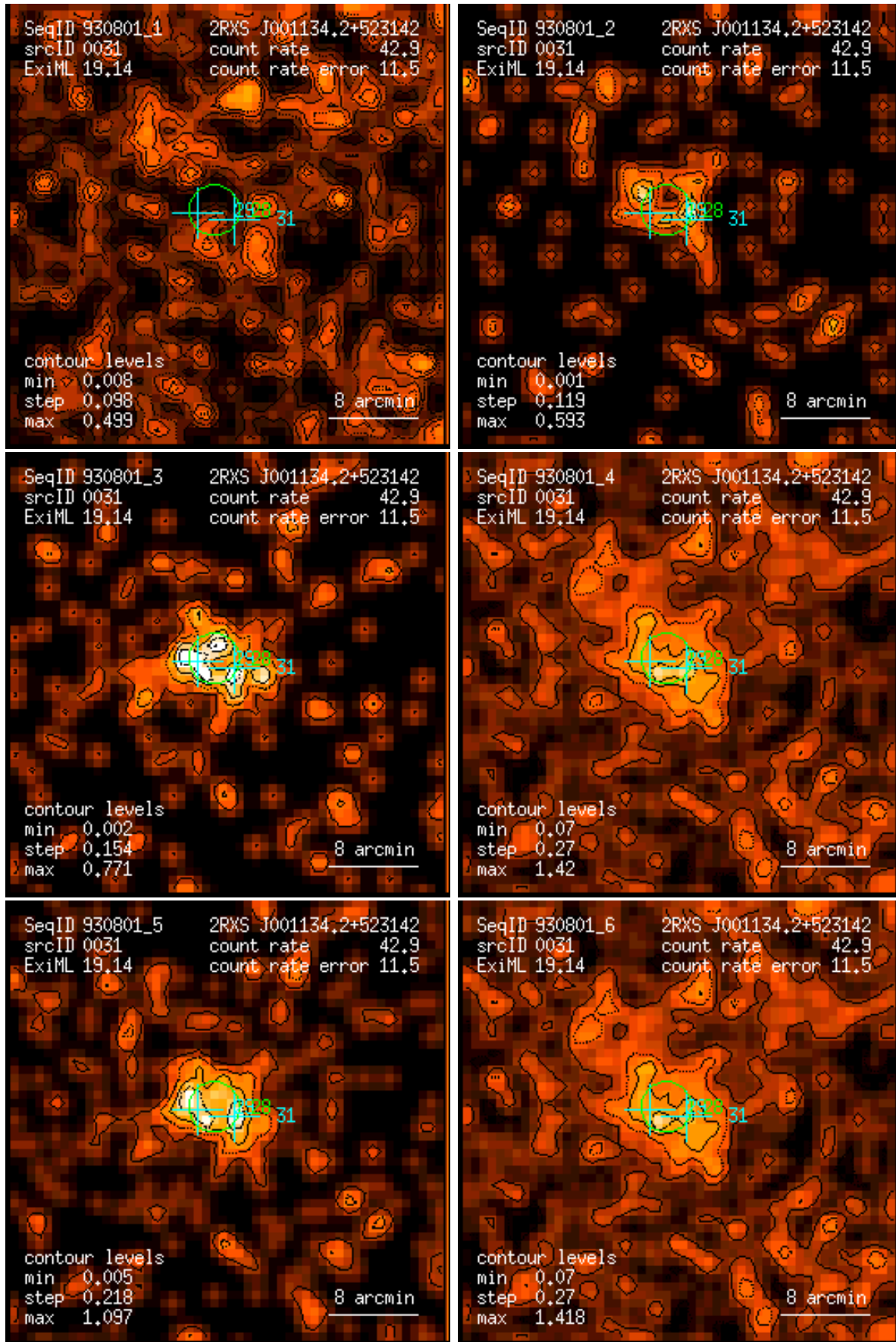
Figure 31: RASS 930801: detection 0031: band rate images, Gaussian filter: (1) PSPC channels 11 – 41, (2) 52 – 90, (3) 91 – 201, (4) 11 – 235, (5) 52 – 201, (6) 11 – 201. Broad band rates in counts/ks. Band rate contour levels in counts/ks/arcmin 2 .
