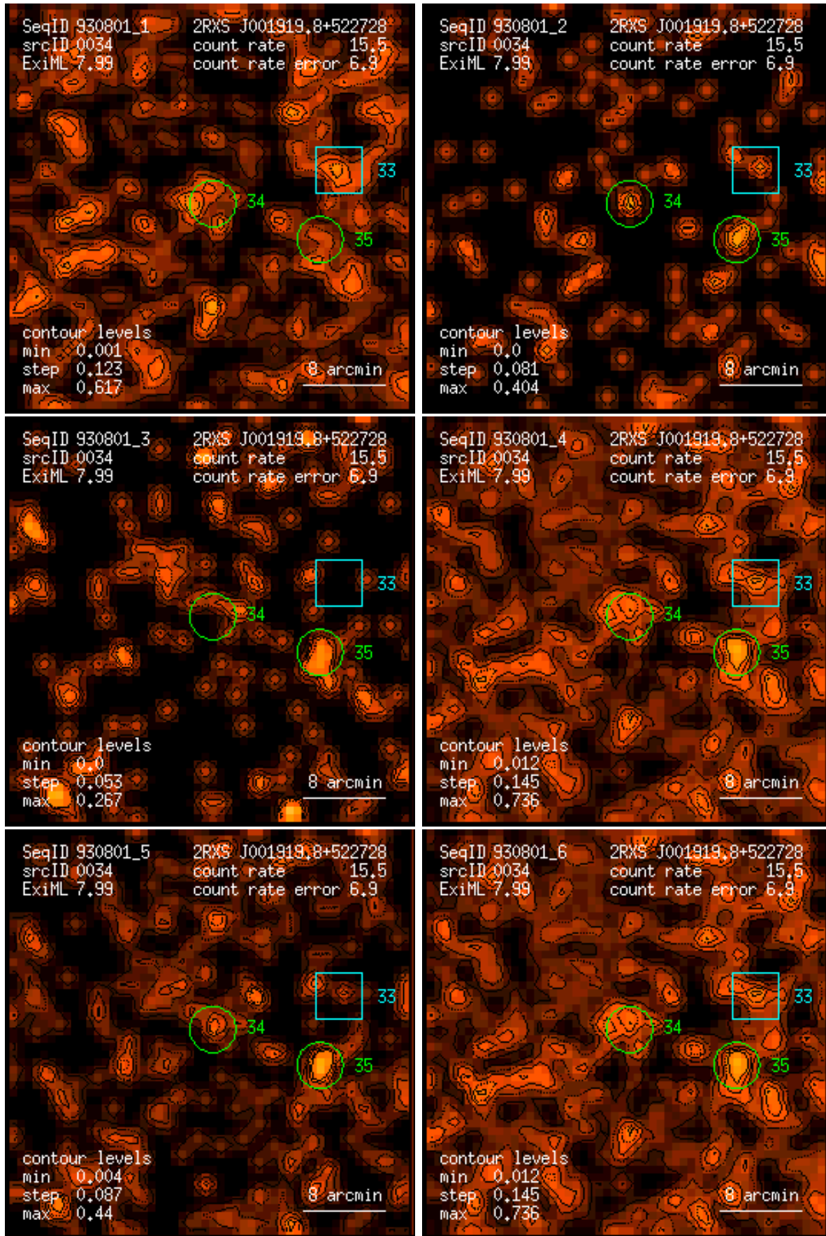
Figure 34: RASS 930801: detection 0034: band rate images, Gaussian filter: (1) PSPC channels 11 – 41, (2) 52 – 90, (3) 91 – 201, (4) 11 – 235, (5) 52 – 201, (6) 11 – 201. Broad band rates in counts/ks. Band rate contour levels in counts/ks/arcmin 2 .
