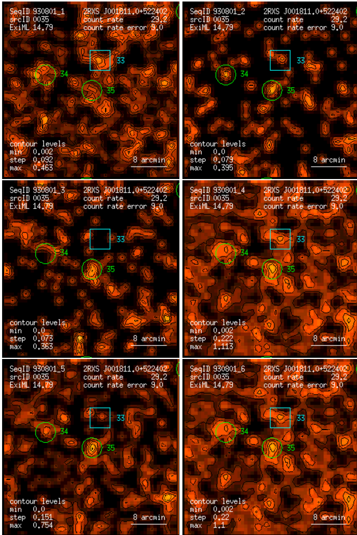
Figure 35: RASS 930801: detection 0035: band rate images, Gaussian filter: (1) PSPC channels 11 – 41, (2) 52 – 90, (3) 91 – 201, (4) 11 – 235, (5) 52 – 201, (6) 11 – 201. Broad band rates in counts/ks. Band rate contour levels in counts/ks/arcmin 2 .
