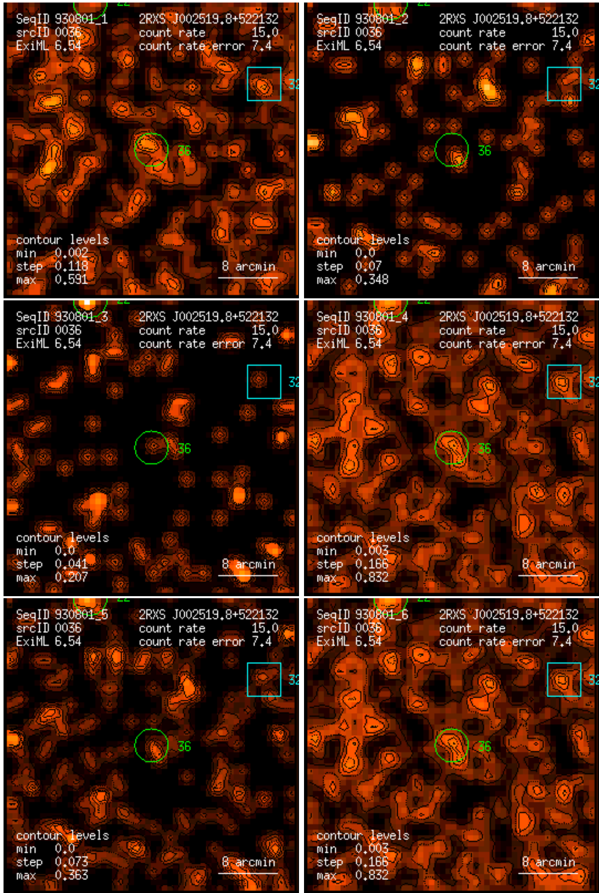
Figure 36: RASS 930801: detection 0036: band rate images, Gaussian filter: (1) PSPC channels 11 – 41, (2) 52 – 90, (3) 91 – 201, (4) 11 – 235, (5) 52 – 201, (6) 11 – 201. Broad band rates in counts/ks. Band rate contour levels in counts/ks/arcmin 2 .
