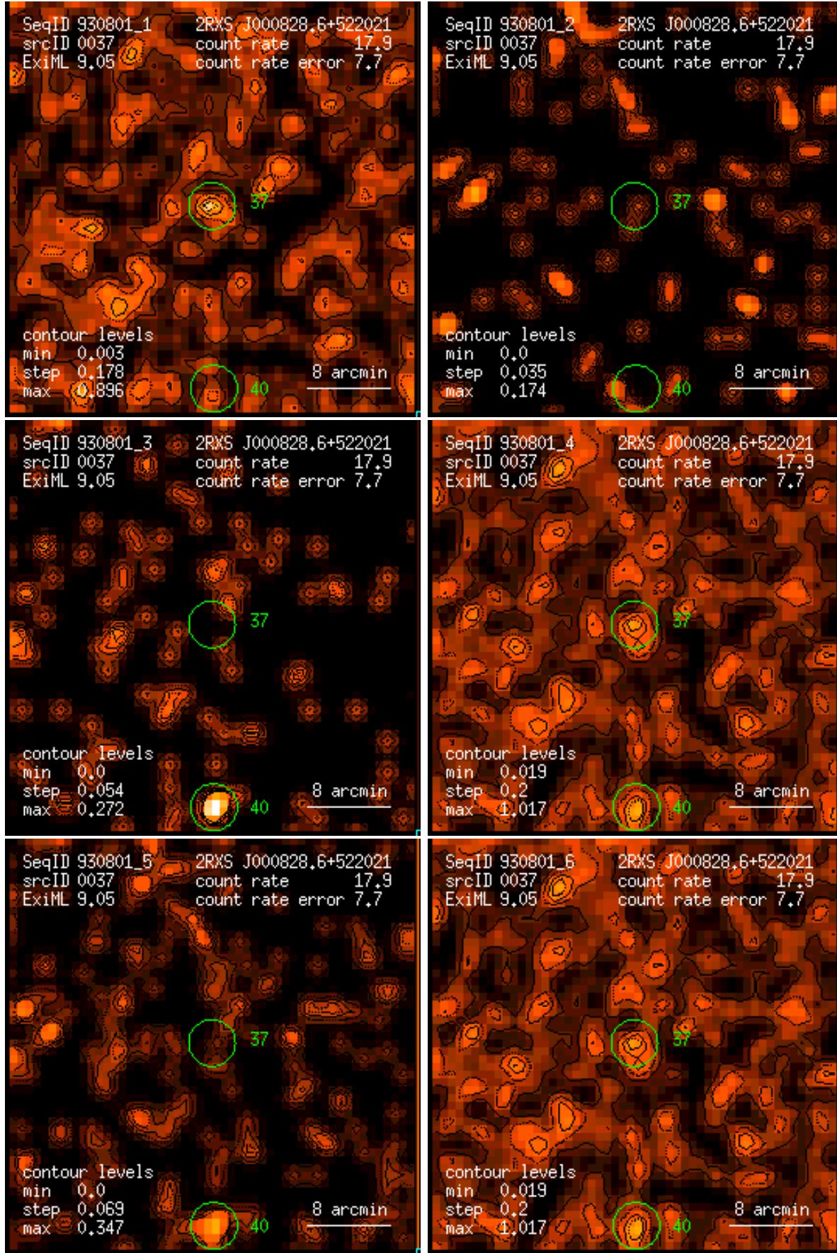
Figure 37: RASS 930801: detection 0037: band rate images, Gaussian filter: (1) PSPC channels 11 – 41, (2) 52 – 90, (3) 91 – 201, (4) 11 – 235, (5) 52 – 201, (6) 11 – 201. Broad band rates in counts/ks. Band rate contour levels in counts/ks/arcmin 2 .
