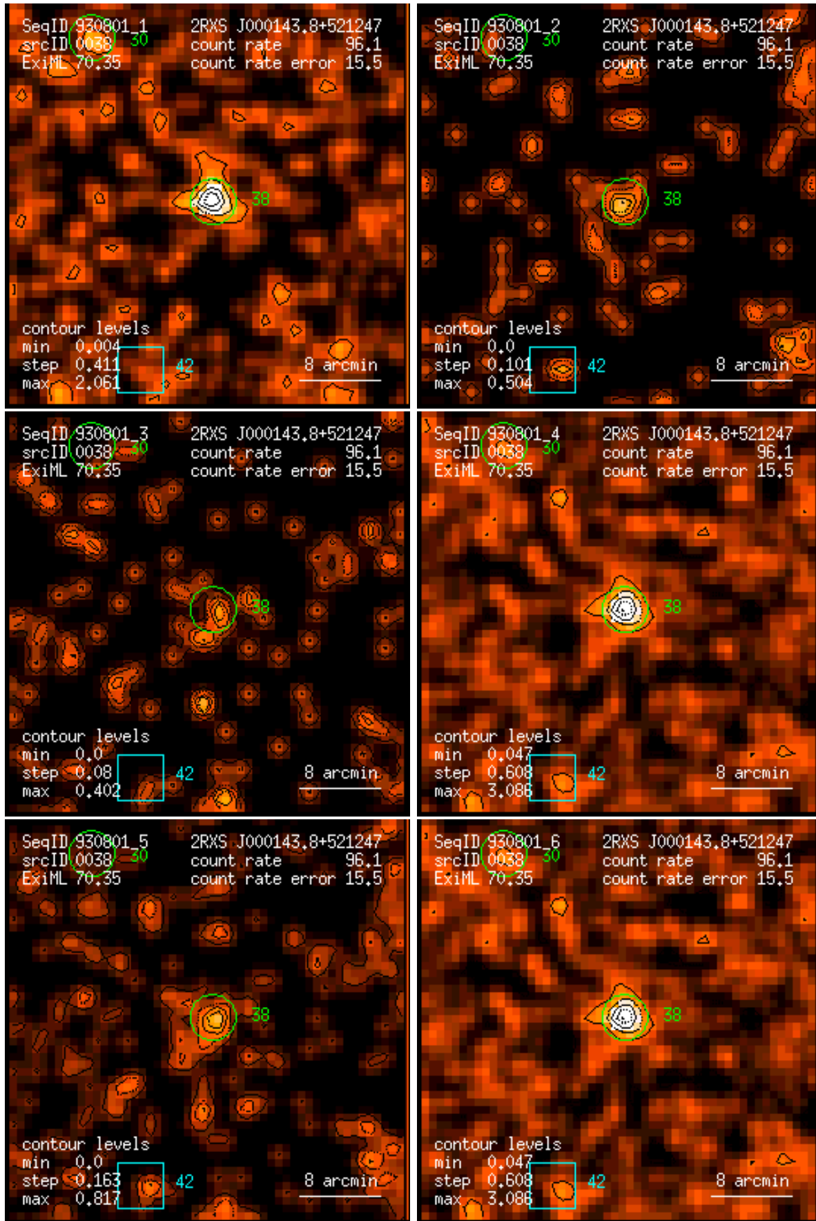
Figure 38: RASS 930801: detection 0038: band rate images, Gaussian filter: (1) PSPC channels 11 – 41, (2) 52 – 90, (3) 91 – 201, (4) 11 – 235, (5) 52 – 201, (6) 11 – 201. Broad band rates in counts/ks. Band rate contour levels in counts/ks/arcmin 2 .
