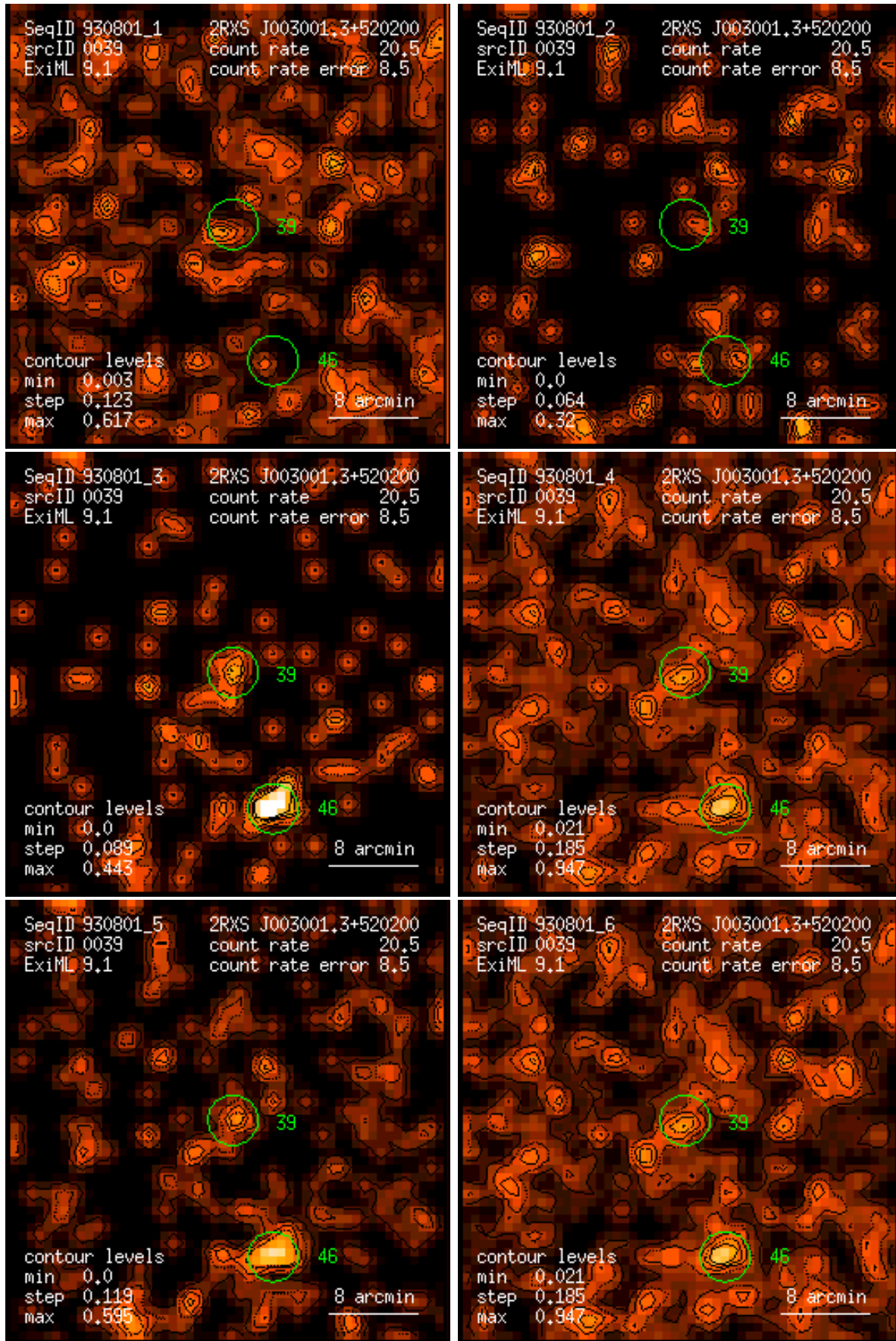
Figure 39: RASS 930801: detection 0039: band rate images, Gaussian filter: (1) PSPC channels 11 – 41, (2) 52 – 90, (3) 91 – 201, (4) 11 – 235, (5) 52 – 201, (6) 11 – 201. Broad band rates in counts/ks. Band rate contour levels in counts/ks/arcmin 2 .
