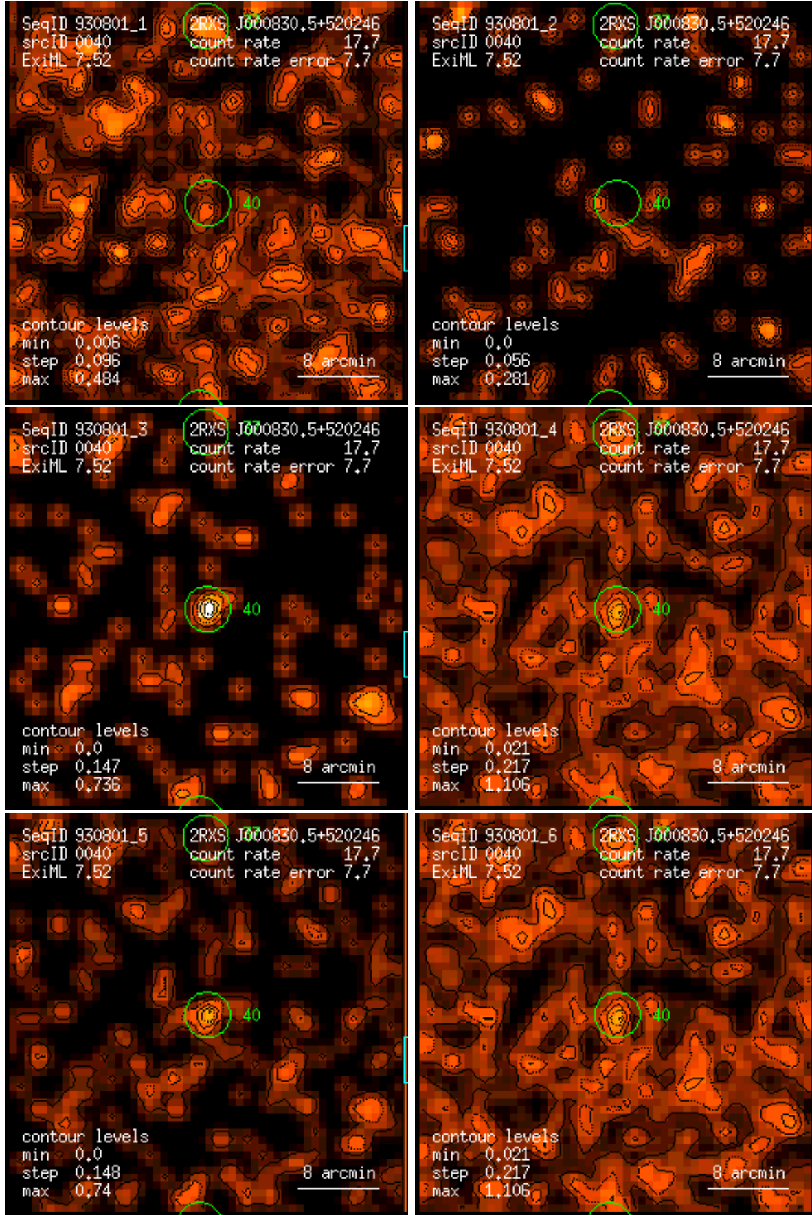
Figure 40: RASS 930801: detection 0040: band rate images, Gaussian filter: (1) PSPC channels 11 – 41, (2) 52 – 90, (3) 91 – 201, (4) 11 – 235, (5) 52 – 201, (6) 11 – 201. Broad band rates in counts/ks. Band rate contour levels in counts/ks/arcmin 2 .
