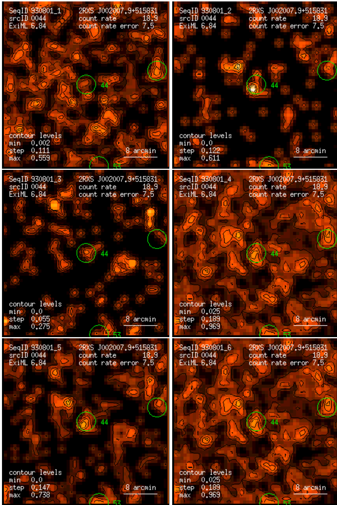
Figure 44: RASS 930801: detection 0044: band rate images, Gaussian filter: (1) PSPC channels 11 – 41, (2) 52 – 90, (3) 91 – 201, (4) 11 – 235, (5) 52 – 201, (6) 11 – 201. Broad band rates in counts/ks. Band rate contour levels in counts/ks/arcmin 2 .
