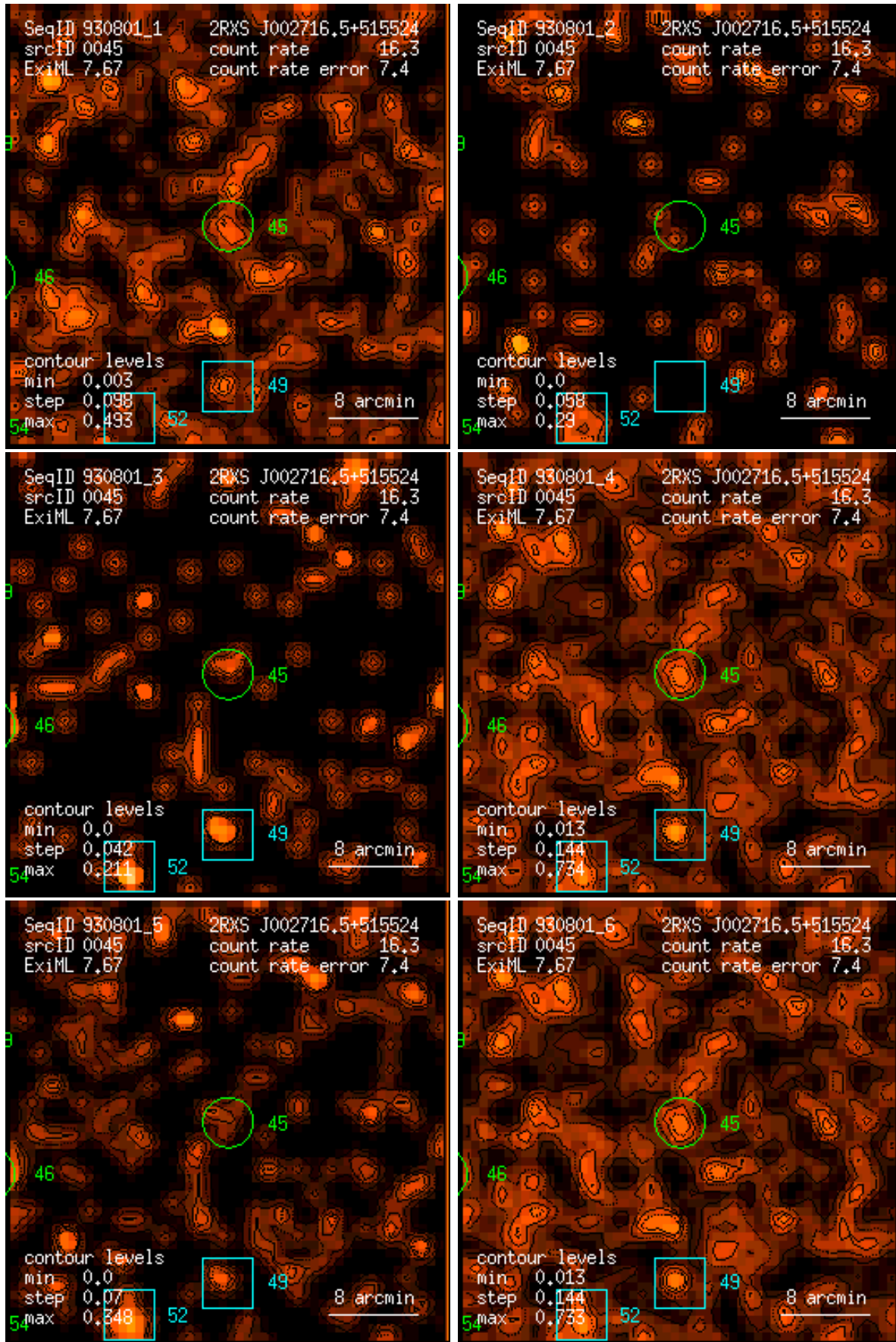
Figure 45: RASS 930801: detection 0045: band rate images, Gaussian filter: (1) PSPC channels 11 – 41, (2) 52 – 90, (3) 91 – 201, (4) 11 – 235, (5) 52 – 201, (6) 11 – 201. Broad band rates in counts/ks. Band rate contour levels in counts/ks/arcmin 2 .
