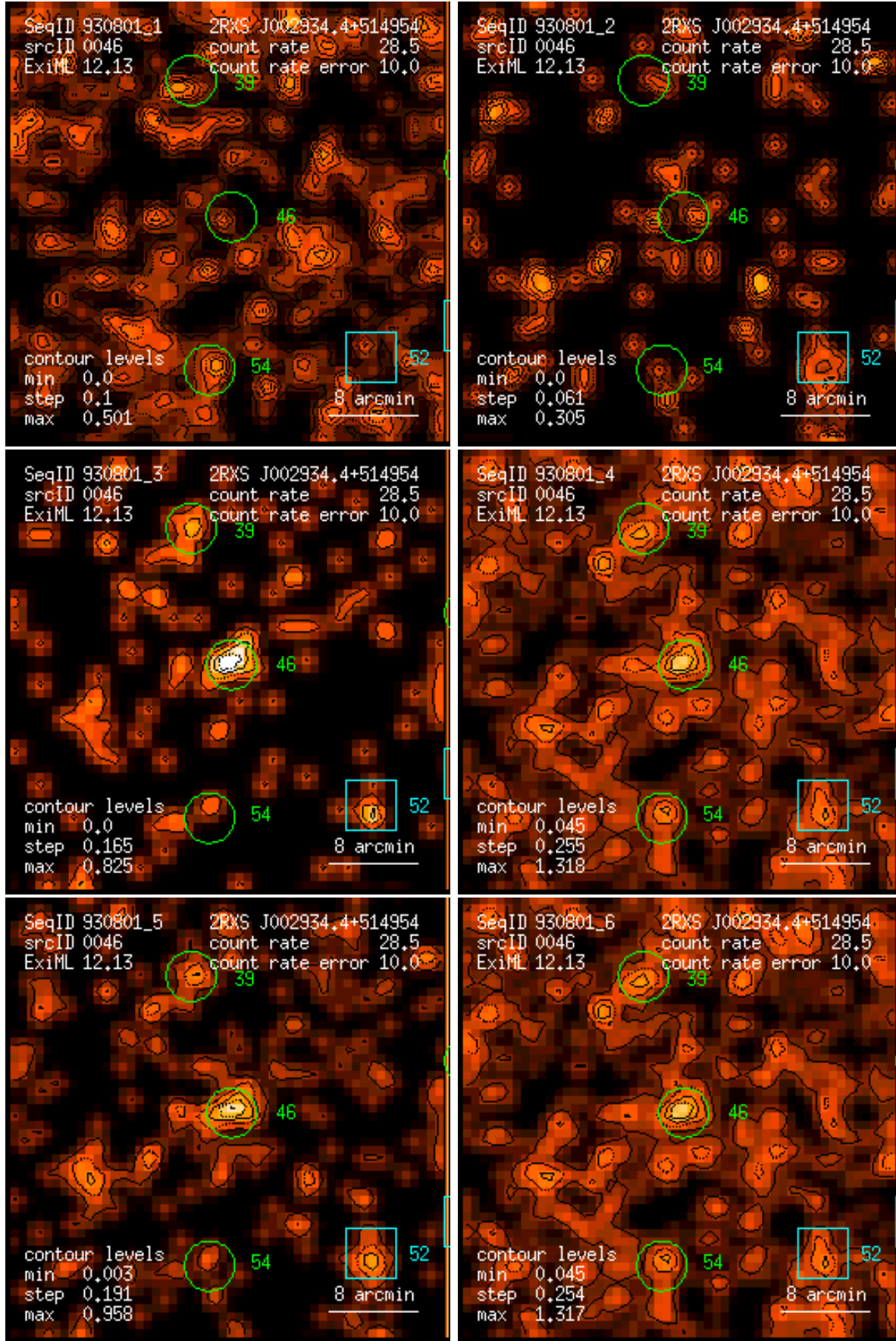
Figure 46: RASS 930801: detection 0046: band rate images, Gaussian filter: (1) PSPC channels 11 – 41, (2) 52 – 90, (3) 91 – 201, (4) 11 – 235, (5) 52 – 201, (6) 11 – 201. Broad band rates in counts/ks. Band rate contour levels in counts/ks/arcmin 2 .
