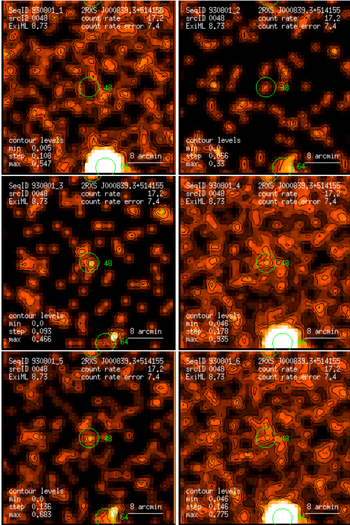
Figure 48: RASS 930801: detection 0048: band rate images, Gaussian filter: (1) PSPC channels 11 – 41, (2) 52 – 90, (3) 91 – 201, (4) 11 – 235, (5) 52 – 201, (6) 11 – 201. Broad band rates in counts/ks. Band rate contour levels in counts/ks/arcmin 2 .
