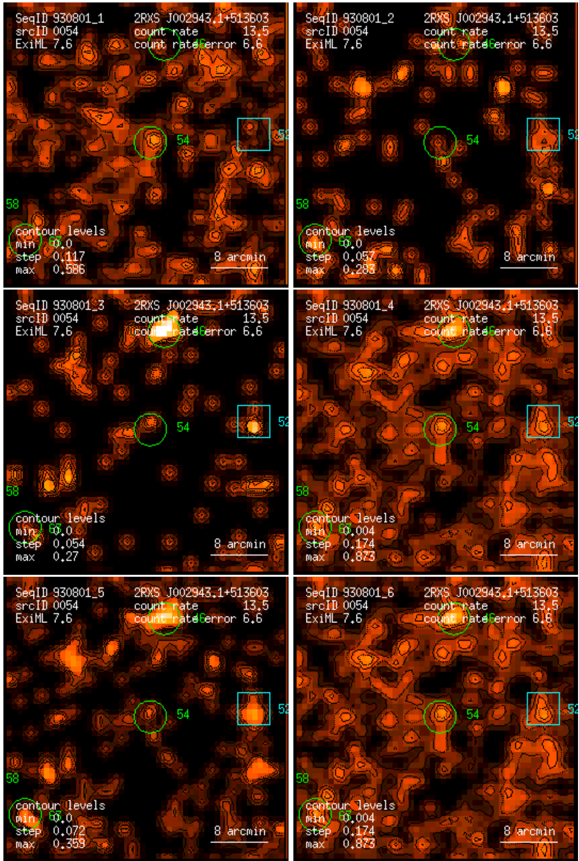
Figure 54: RASS 930801: detection 0054: band rate images, Gaussian filter: (1) PSPC channels 11 – 41, (2) 52 – 90, (3) 91 – 201, (4) 11 – 235, (5) 52 – 201, (6) 11 – 201. Broad band rates in counts/ks. Band rate contour levels in counts/ks/arcmin 2 .
