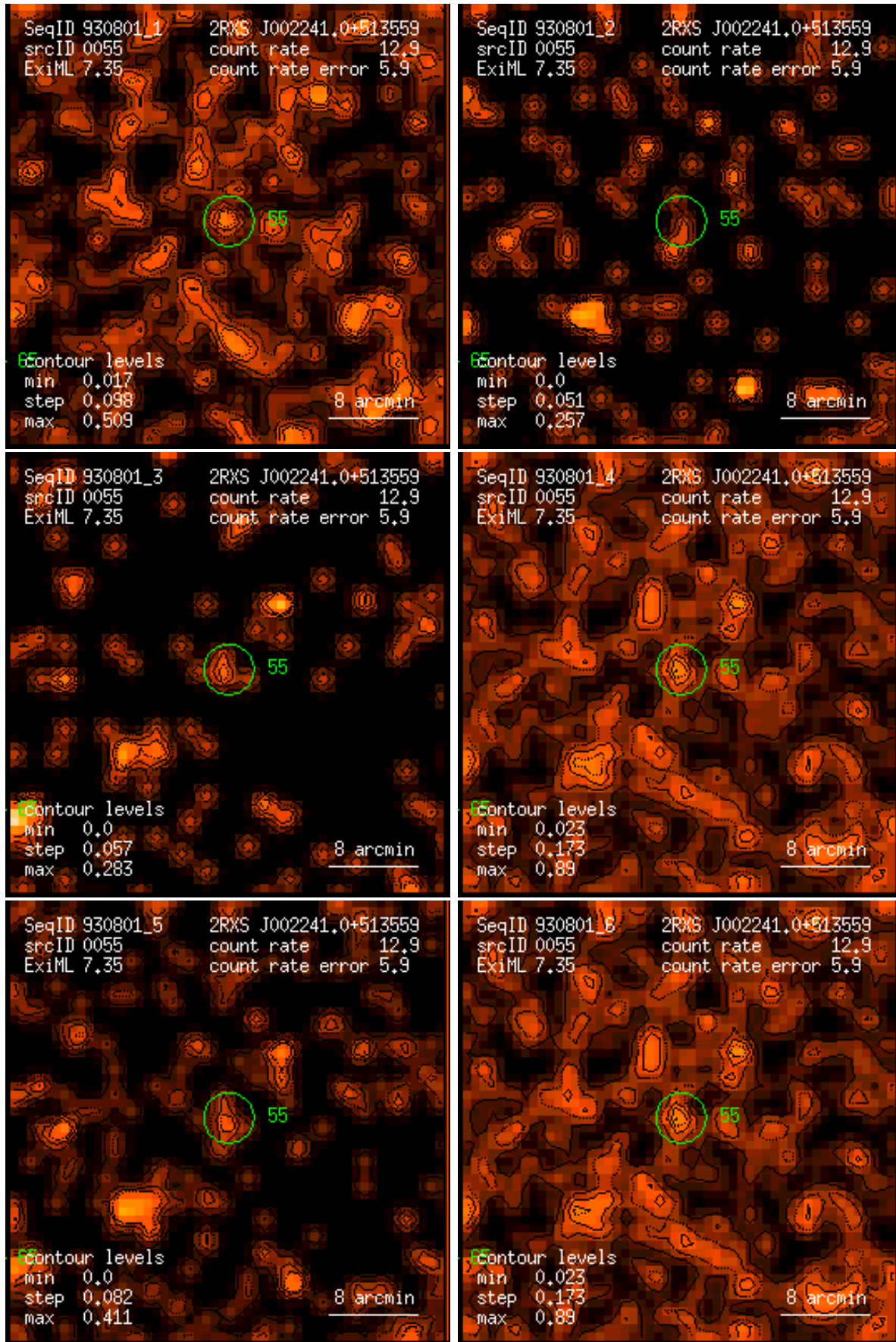
Figure 55: RASS 930801: detection 0055: band rate images, Gaussian filter: (1) PSPC channels 11 – 41, (2) 52 – 90, (3) 91 – 201, (4) 11 – 235, (5) 52 – 201, (6) 11 – 201. Broad band rates in counts/ks. Band rate contour levels in counts/ks/arcmin 2 .
