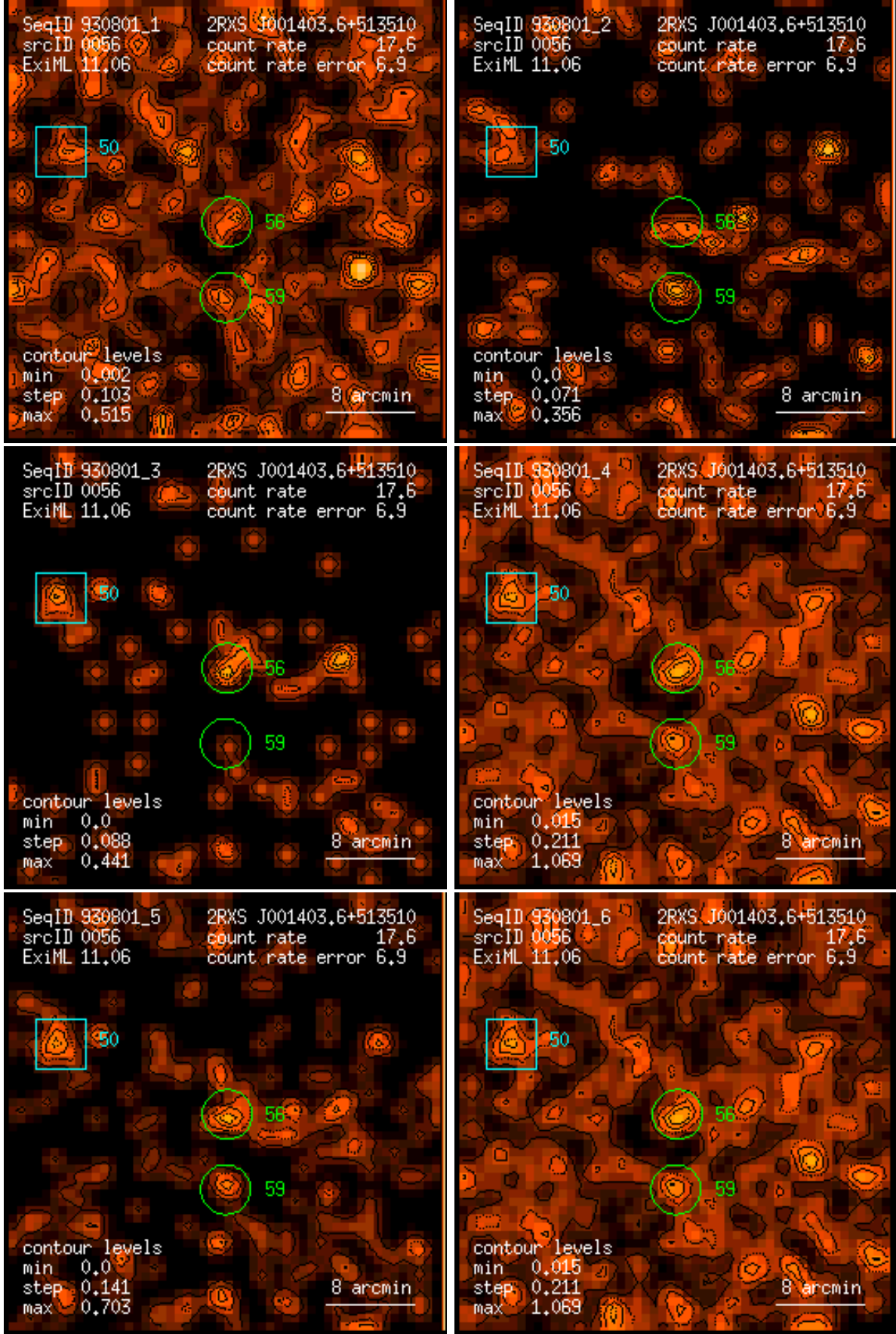
Figure 56: RASS 930801: detection 0056: band rate images, Gaussian filter: (1) PSPC channels 11 – 41, (2) 52 – 90, (3) 91 – 201, (4) 11 – 235, (5) 52 – 201, (6) 11 – 201. Broad band rates in counts/ks. Band rate contour levels in counts/ks/arcmin 2 .
