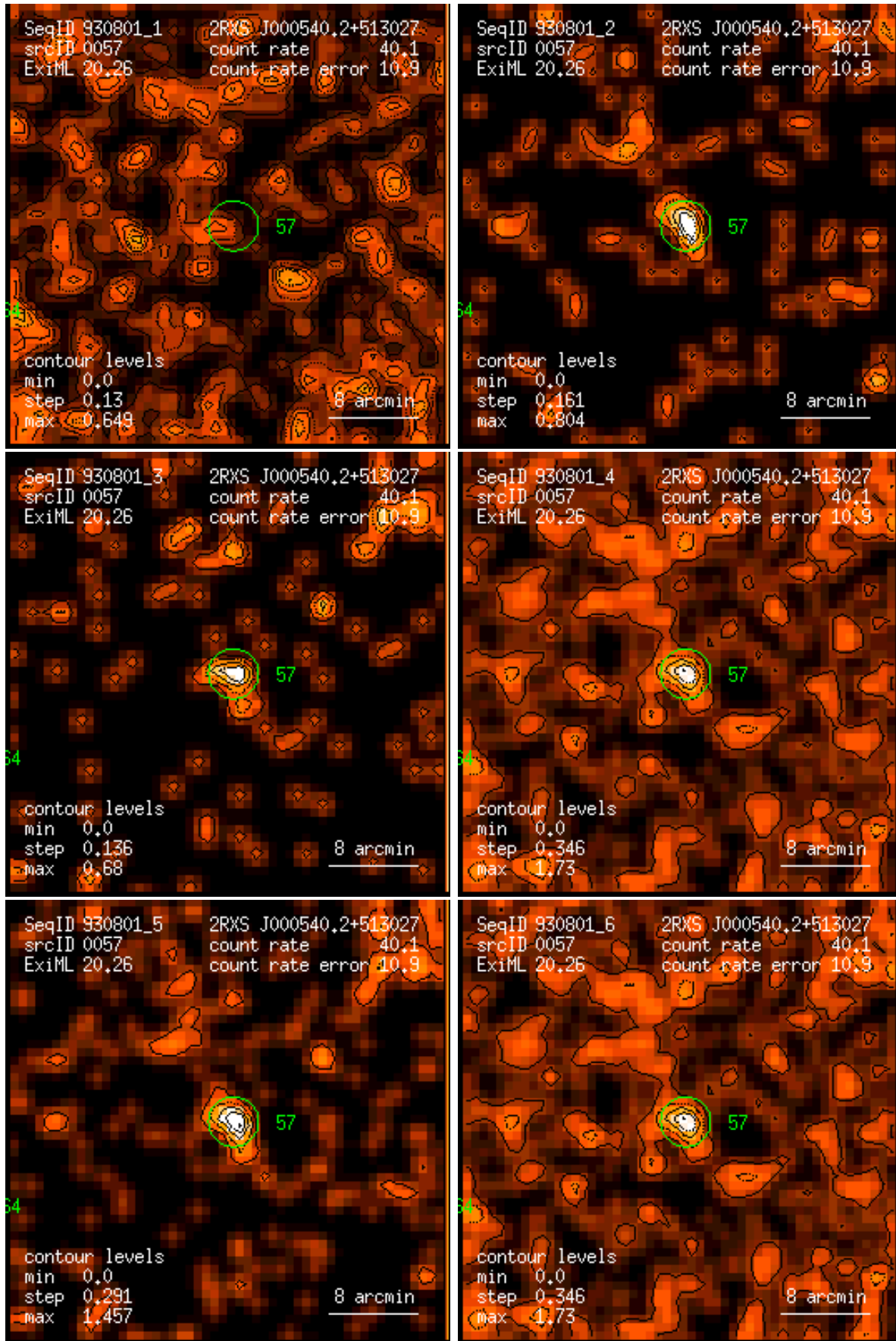
Figure 57: RASS 930801: detection 0057: band rate images, Gaussian filter: (1) PSPC channels 11 – 41, (2) 52 – 90, (3) 91 – 201, (4) 11 – 235, (5) 52 – 201, (6) 11 – 201. Broad band rates in counts/ks. Band rate contour levels in counts/ks/arcmin 2 .
