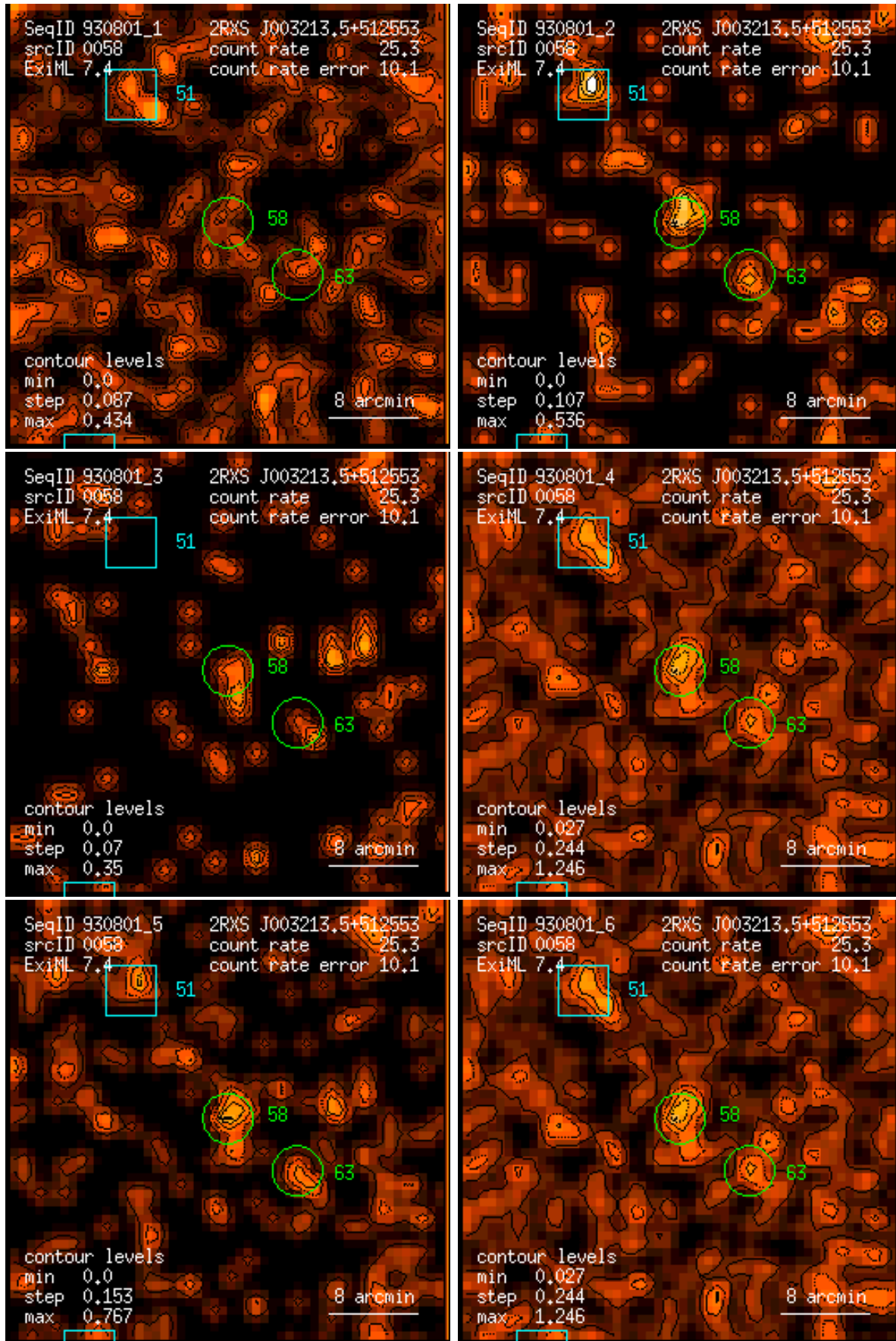
Figure 58: RASS 930801: detection 0058: band rate images, Gaussian filter: (1) PSPC channels 11 – 41, (2) 52 – 90, (3) 91 – 201, (4) 11 – 235, (5) 52 – 201, (6) 11 – 201. Broad band rates in counts/ks. Band rate contour levels in counts/ks/arcmin 2 .
