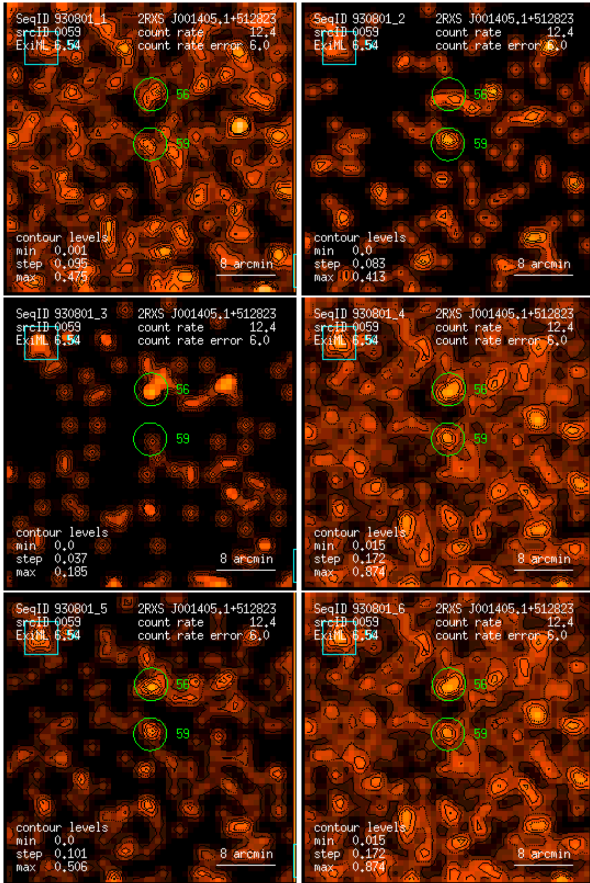
Figure 59: RASS 930801: detection 0059: band rate images, Gaussian filter: (1) PSPC channels 11 – 41, (2) 52 – 90, (3) 91 – 201, (4) 11 – 235, (5) 52 – 201, (6) 11 – 201. Broad band rates in counts/ks. Band rate contour levels in counts/ks/arcmin 2 .
