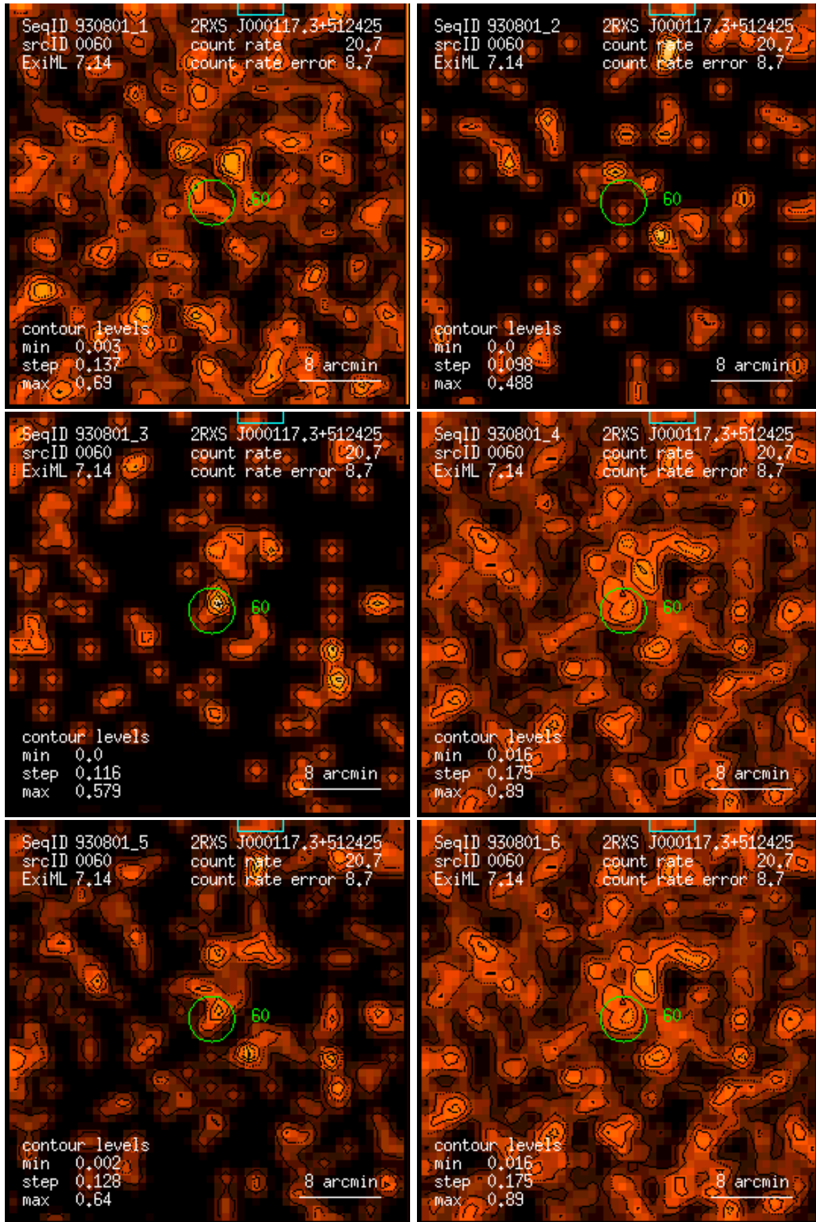
Figure 60: RASS 930801: detection 0060: band rate images, Gaussian filter: (1) PSPC channels 11 – 41, (2) 52 – 90, (3) 91 – 201, (4) 11 – 235, (5) 52 – 201, (6) 11 – 201. Broad band rates in counts/ks. Band rate contour levels in counts/ks/arcmin 2 .
