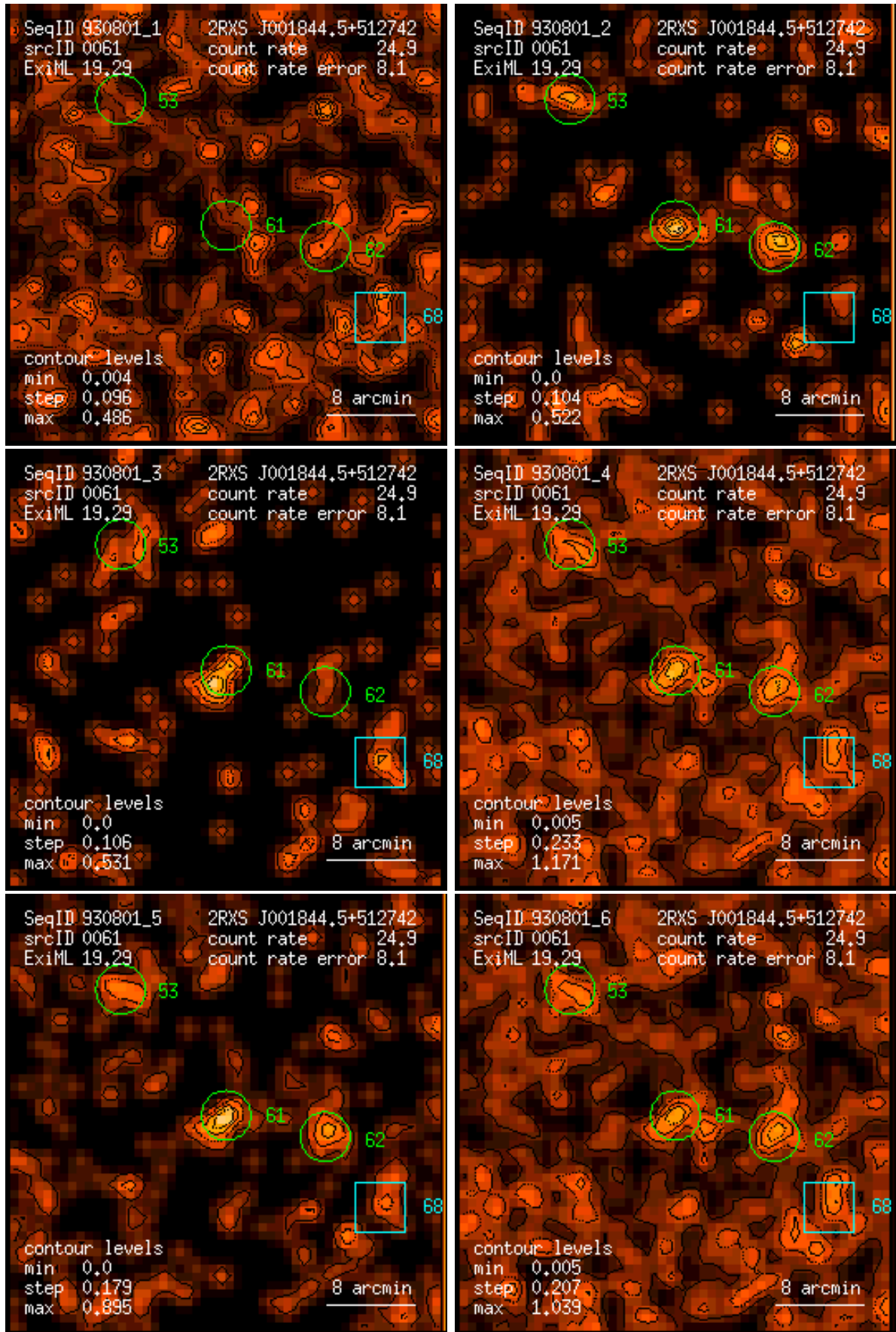
Figure 61: RASS 930801: detection 0061: band rate images, Gaussian filter: (1) PSPC channels 11 – 41, (2) 52 – 90, (3) 91 – 201, (4) 11 – 235, (5) 52 – 201, (6) 11 – 201. Broad band rates in counts/ks. Band rate contour levels in counts/ks/arcmin 2 .
