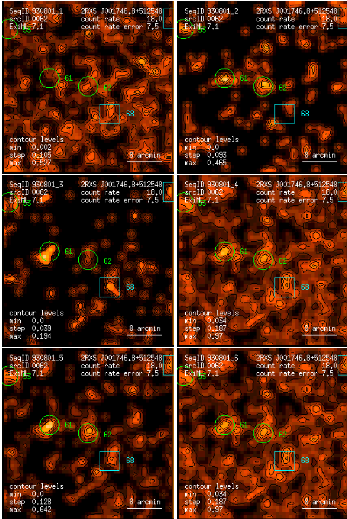
Figure 62: RASS 930801: detection 0062: band rate images, Gaussian filter: (1) PSPC channels 11 – 41, (2) 52 – 90, (3) 91 – 201, (4) 11 – 235, (5) 52 – 201, (6) 11 – 201. Broad band rates in counts/ks. Band rate contour levels in counts/ks/arcmin 2 .
