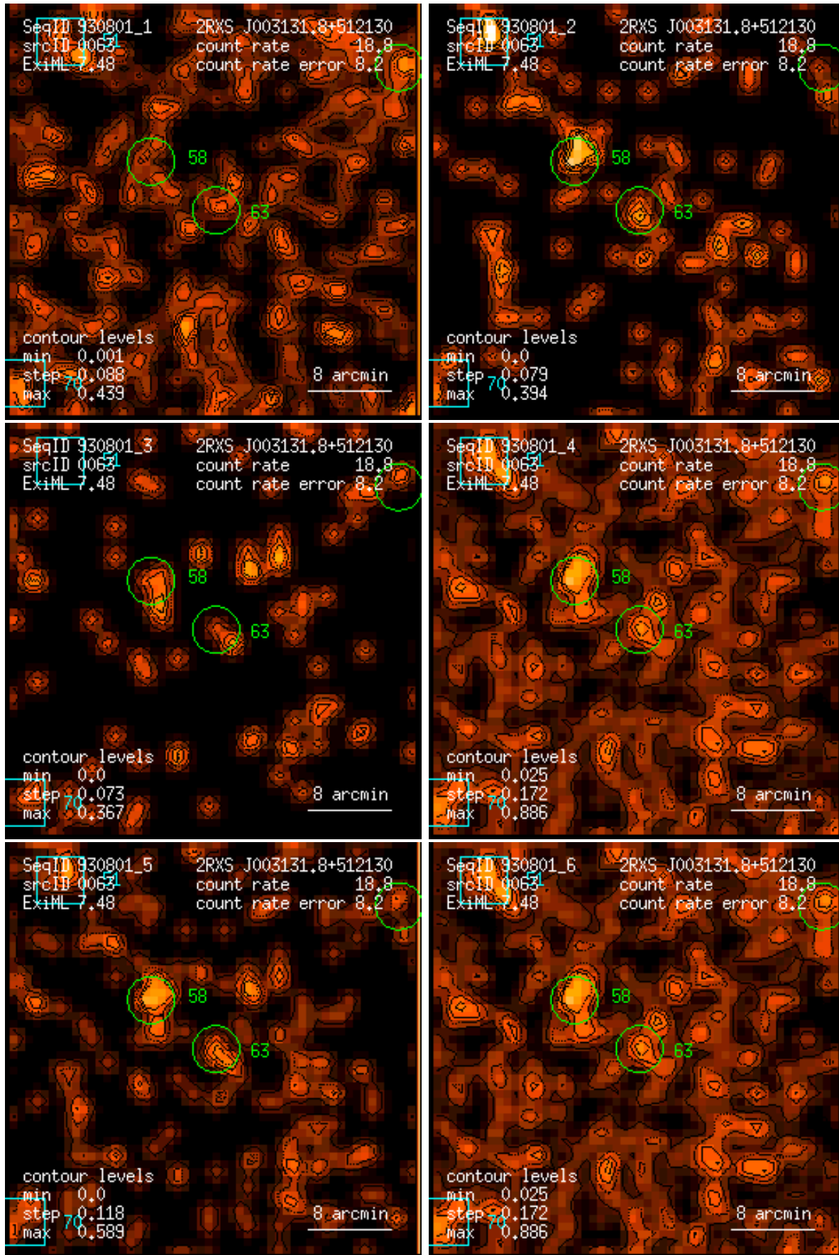
Figure 63: RASS 930801: detection 0063: band rate images, Gaussian filter: (1) PSPC channels 11 – 41, (2) 52 – 90, (3) 91 – 201, (4) 11 – 235, (5) 52 – 201, (6) 11 – 201. Broad band rates in counts/ks. Band rate contour levels in counts/ks/arcmin 2 .
