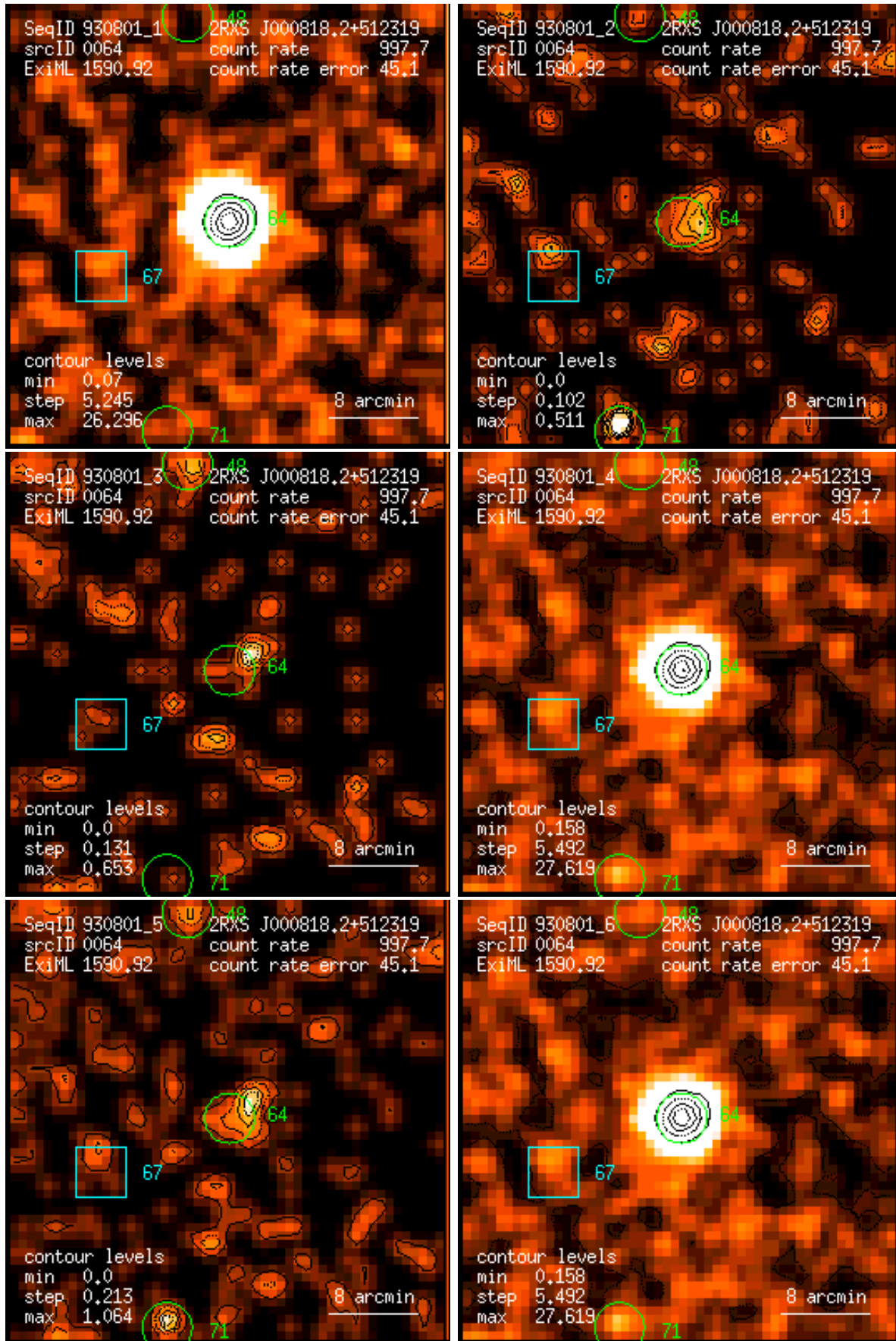
Figure 64: RASS 930801: detection 0064: band rate images, Gaussian filter: (1) PSPC channels 11 – 41, (2) 52 – 90, (3) 91 – 201, (4) 11 – 235, (5) 52 – 201, (6) 11 – 201. Broad band rates in counts/ks. Band rate contour levels in counts/ks/arcmin 2 .
