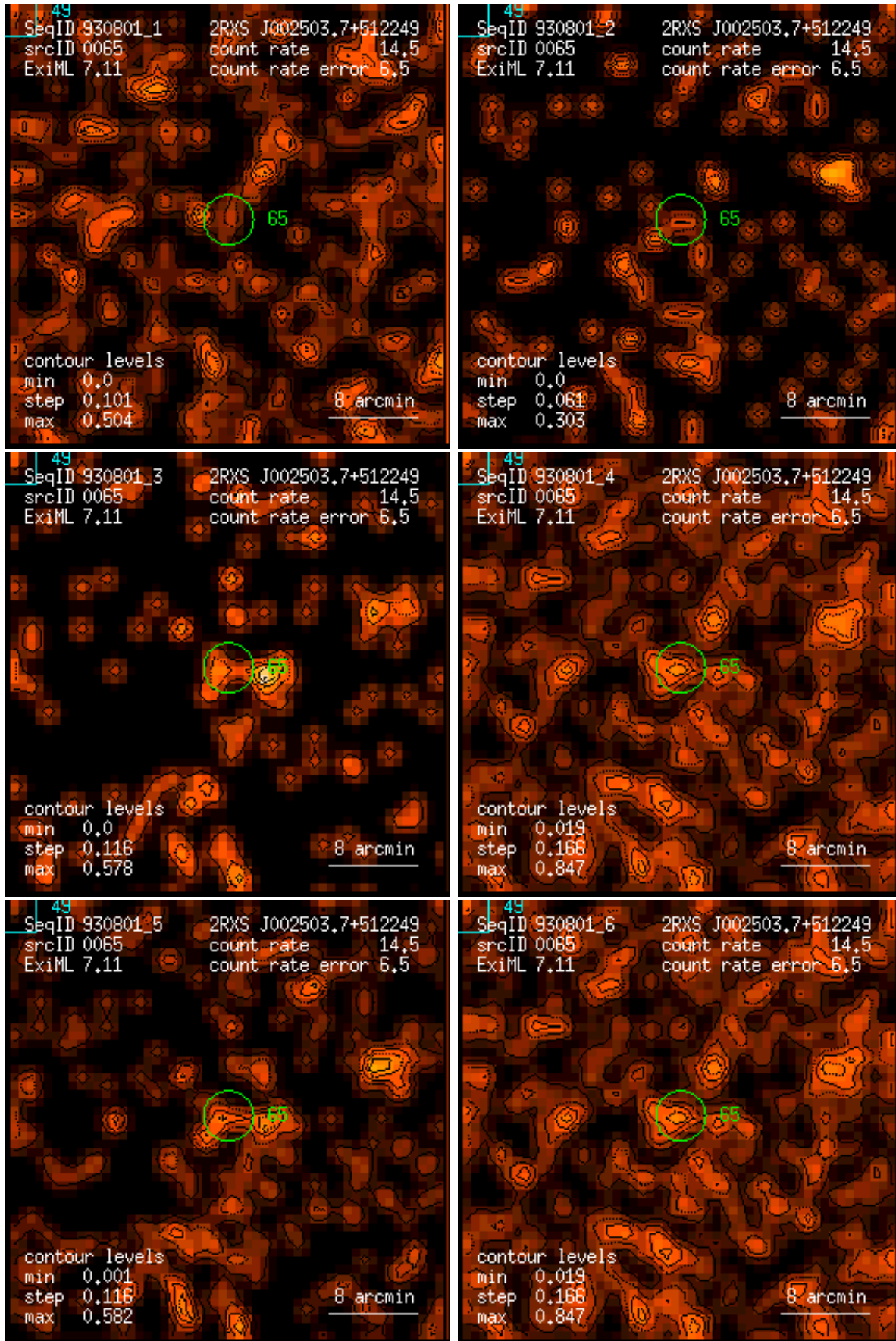
Figure 65: RASS 930801: detection 0065: band rate images, Gaussian filter: (1) PSPC channels 11 – 41, (2) 52 – 90, (3) 91 – 201, (4) 11 – 235, (5) 52 – 201, (6) 11 – 201. Broad band rates in counts/ks. Band rate contour levels in counts/ks/arcmin 2 .
