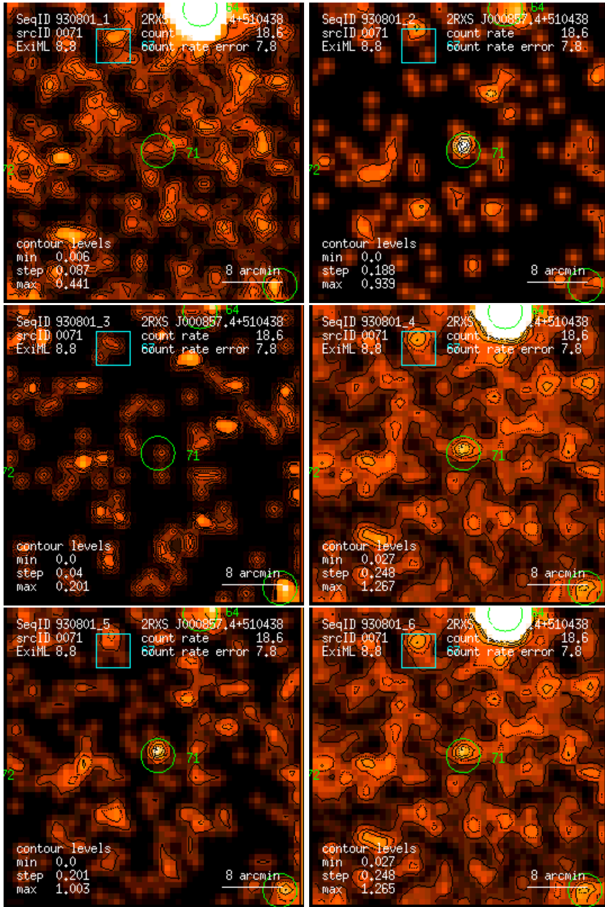
Figure 71: RASS 930801: detection 0071: band rate images, Gaussian filter: (1) PSPC channels 11 – 41, (2) 52 – 90, (3) 91 – 201, (4) 11 – 235, (5) 52 – 201, (6) 11 – 201. Broad band rates in counts/ks. Band rate contour levels in counts/ks/arcmin 2 .
