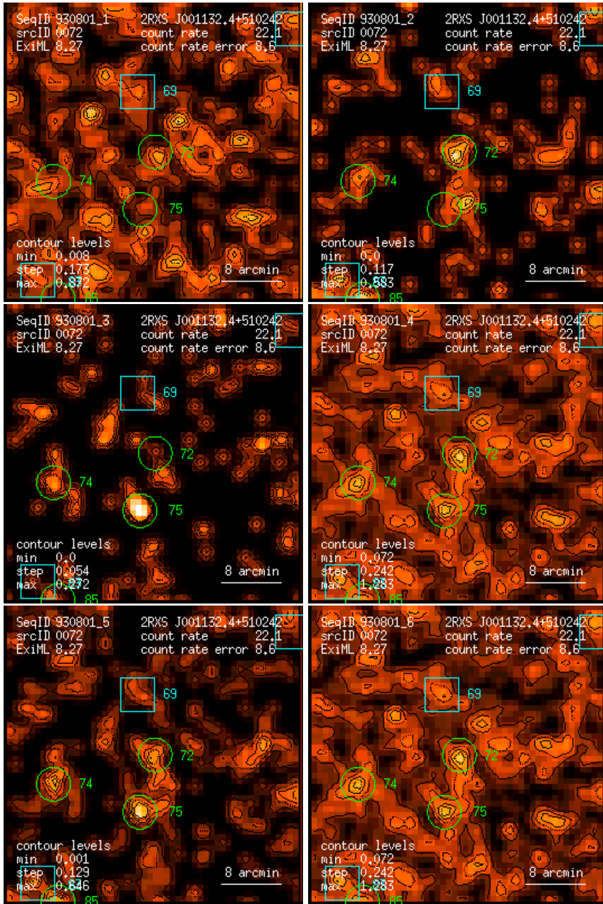
Figure 72: RASS 930801: detection 0072: band rate images, Gaussian filter: (1) PSPC channels 11 – 41, (2) 52 – 90, (3) 91 – 201, (4) 11 – 235, (5) 52 – 201, (6) 11 – 201. Broad band rates in counts/ks. Band rate contour levels in counts/ks/arcmin 2 .
