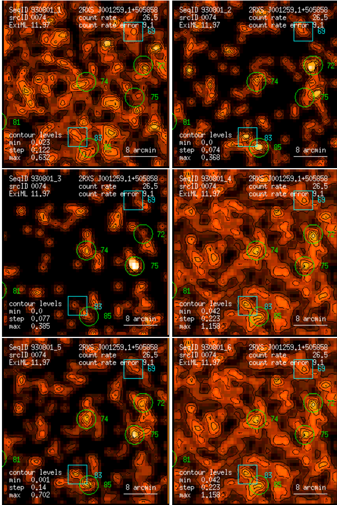
Figure 74: RASS 930801: detection 0074: band rate images, Gaussian filter: (1) PSPC channels 11 – 41, (2) 52 – 90, (3) 91 – 201, (4) 11 – 235, (5) 52 – 201, (6) 11 – 201. Broad band rates in counts/ks. Band rate contour levels in counts/ks/arcmin 2 .
