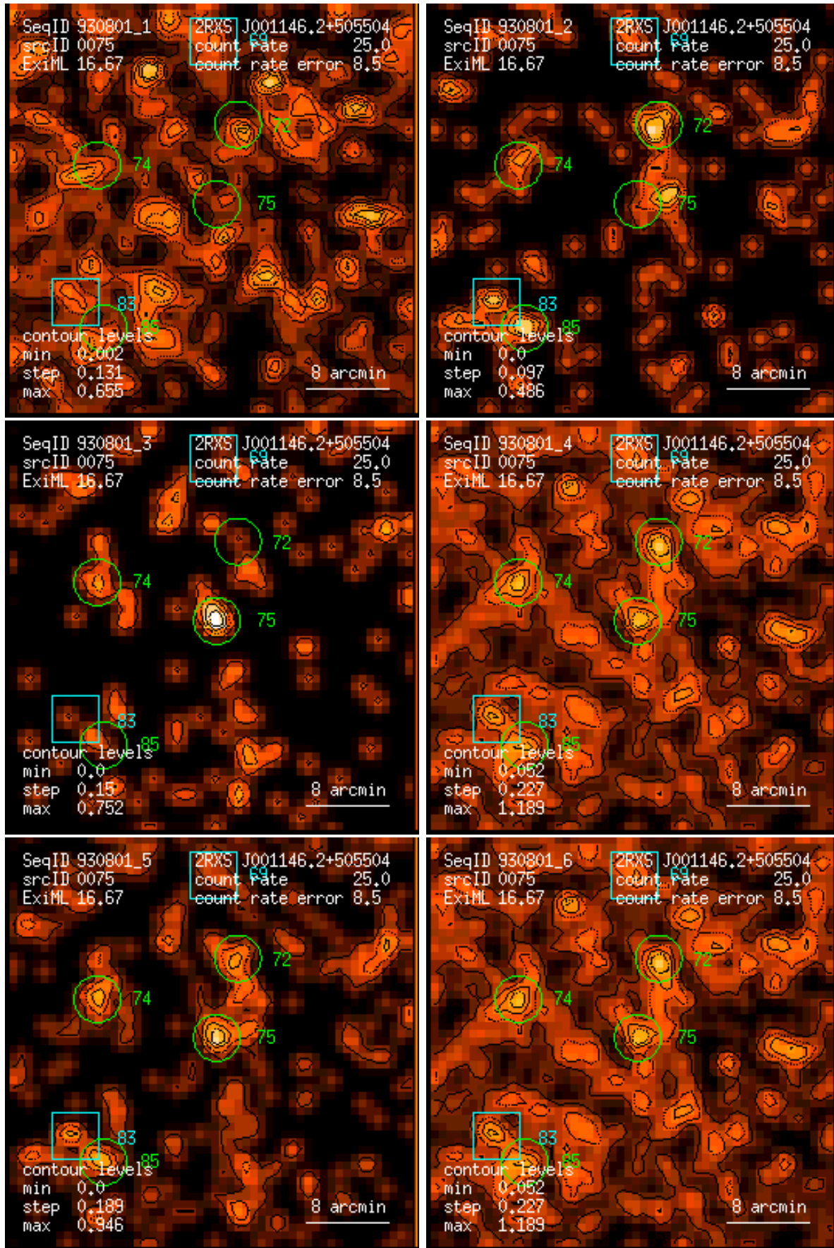
Figure 75: RASS 930801: detection 0075: band rate images, Gaussian filter: (1) PSPC channels 11 – 41, (2) 52 – 90, (3) 91 – 201, (4) 11 – 235, (5) 52 – 201, (6) 11 – 201. Broad band rates in counts/ks. Band rate contour levels in counts/ks/arcmin 2 .
