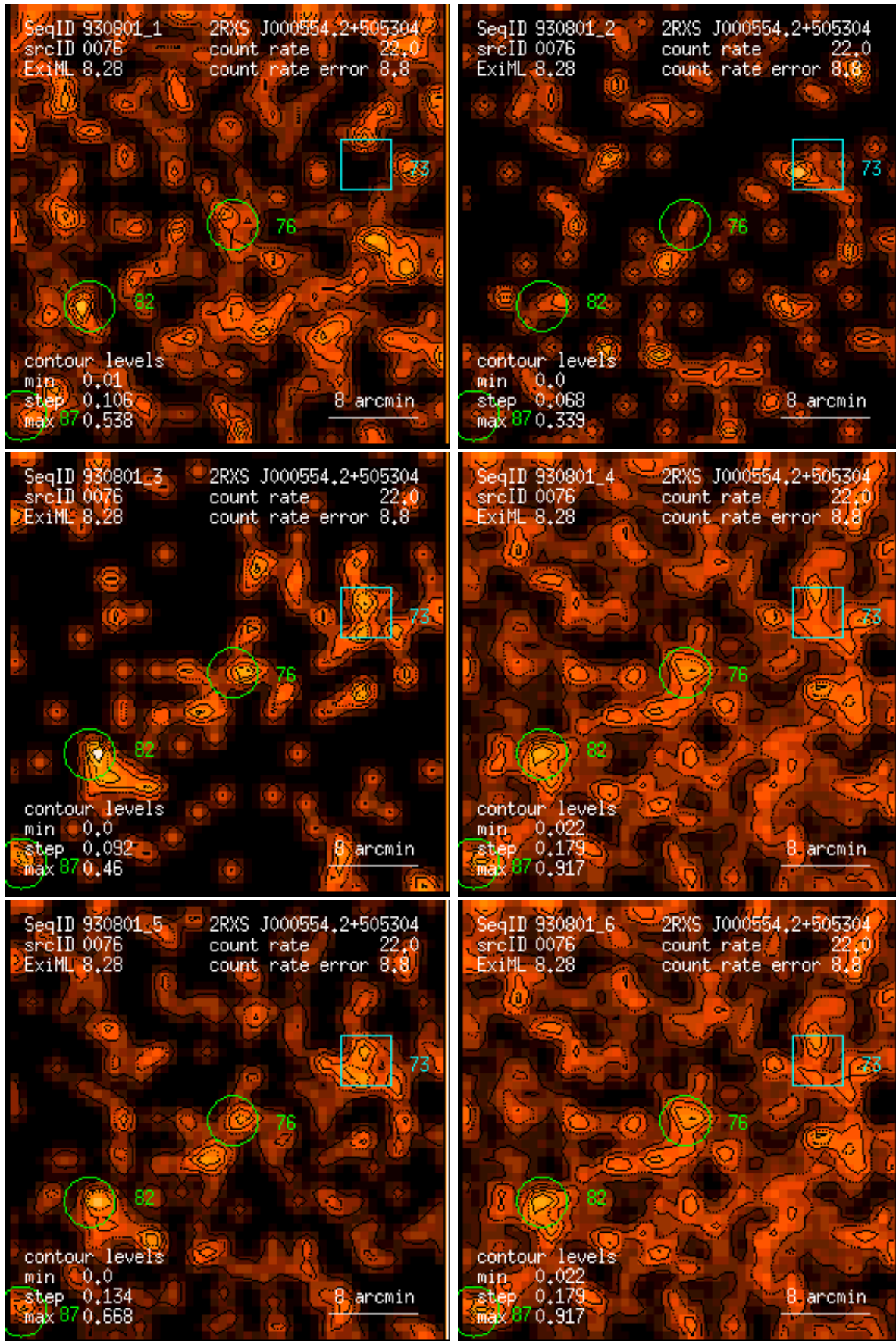
Figure 76: RASS 930801: detection 0076: band rate images, Gaussian filter: (1) PSPC channels 11 – 41, (2) 52 – 90, (3) 91 – 201, (4) 11 – 235, (5) 52 – 201, (6) 11 – 201. Broad band rates in counts/ks. Band rate contour levels in counts/ks/arcmin 2 .
