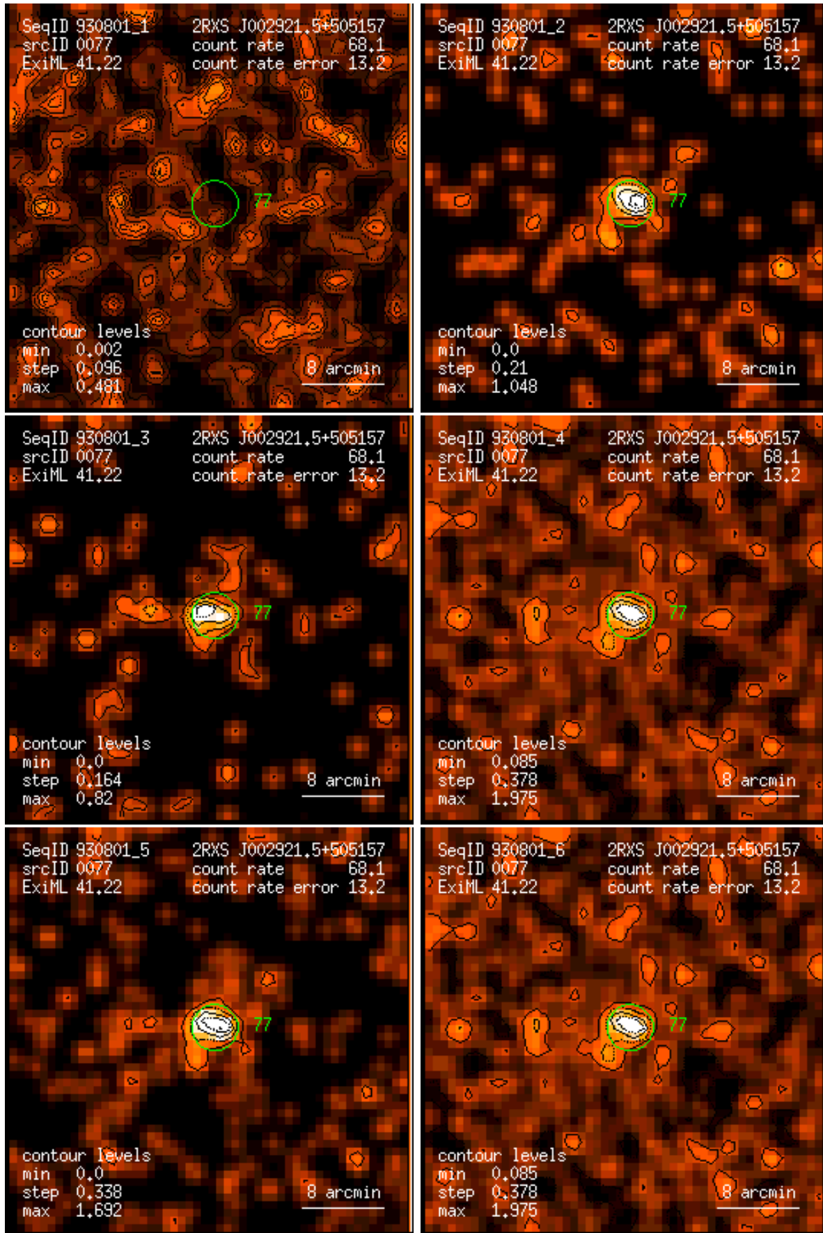
Figure 77: RASS 930801: detection 0077: band rate images, Gaussian filter: (1) PSPC channels 11 – 41, (2) 52 – 90, (3) 91 – 201, (4) 11 – 235, (5) 52 – 201, (6) 11 – 201. Broad band rates in counts/ks. Band rate contour levels in counts/ks/arcmin 2 .
