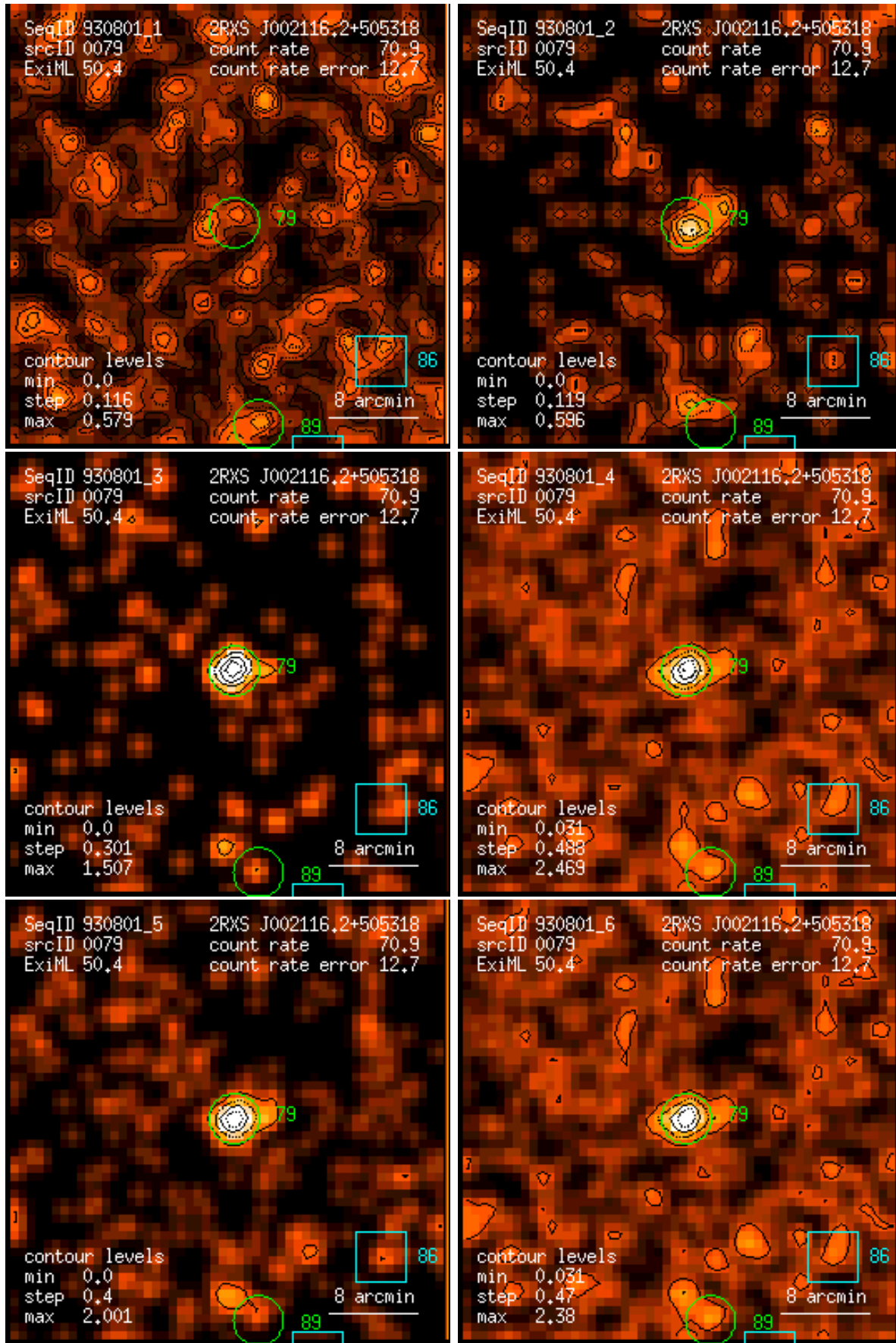
Figure 79: RASS 930801: detection 0079: band rate images, Gaussian filter: (1) PSPC channels 11 – 41, (2) 52 – 90, (3) 91 – 201, (4) 11 – 235, (5) 52 – 201, (6) 11 – 201. Broad band rates in counts/ks. Band rate contour levels in counts/ks/arcmin 2 .
