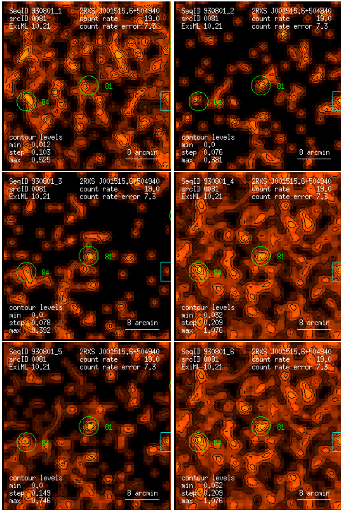
Figure 81: RASS 930801: detection 0081: band rate images, Gaussian filter: (1) PSPC channels 11 – 41, (2) 52 – 90, (3) 91 – 201, (4) 11 – 235, (5) 52 – 201, (6) 11 – 201. Broad band rates in counts/ks. Band rate contour levels in counts/ks/arcmin 2 .
