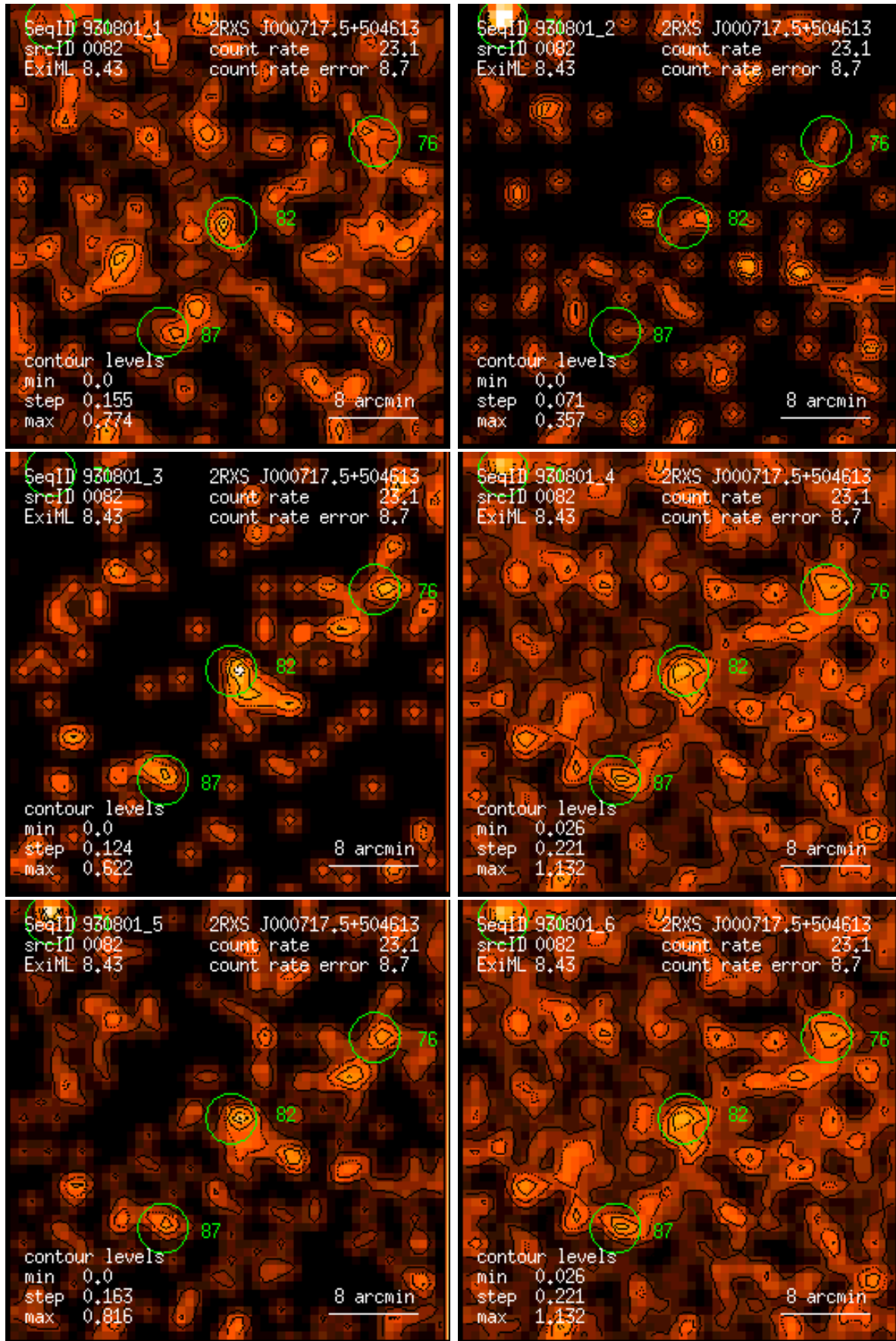
Figure 82: RASS 930801: detection 0082: band rate images, Gaussian filter: (1) PSPC channels 11 – 41, (2) 52 – 90, (3) 91 – 201, (4) 11 – 235, (5) 52 – 201, (6) 11 – 201. Broad band rates in counts/ks. Band rate contour levels in counts/ks/arcmin 2 .
