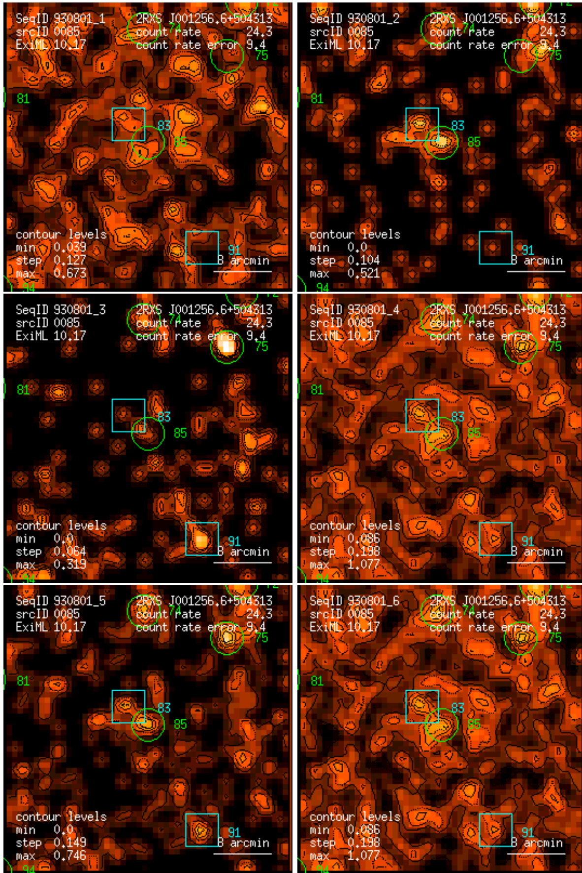
Figure 85: RASS 930801: detection 0085: band rate images, Gaussian filter: (1) PSPC channels 11 – 41, (2) 52 – 90, (3) 91 – 201, (4) 11 – 235, (5) 52 – 201, (6) 11 – 201. Broad band rates in counts/ks. Band rate contour levels in counts/ks/arcmin 2 .
