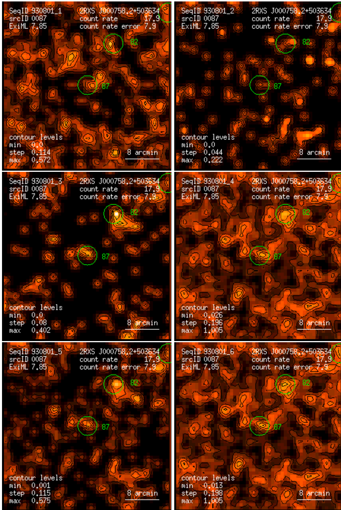
Figure 87: RASS 930801: detection 0087: band rate images, Gaussian filter: (1) PSPC channels 11 – 41, (2) 52 – 90, (3) 91 – 201, (4) 11 – 235, (5) 52 – 201, (6) 11 – 201. Broad band rates in counts/ks. Band rate contour levels in counts/ks/arcmin 2 .
