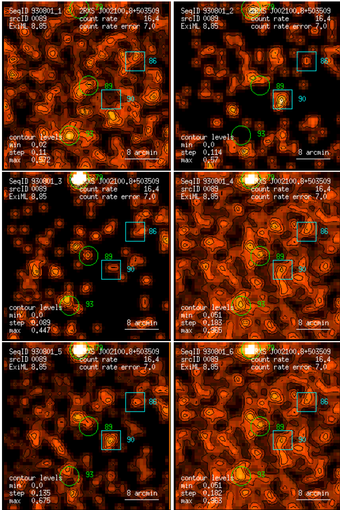
Figure 89: RASS 930801: detection 0089: band rate images, Gaussian filter: (1) PSPC channels 11 – 41, (2) 52 – 90, (3) 91 – 201, (4) 11 – 235, (5) 52 – 201, (6) 11 – 201. Broad band rates in counts/ks. Band rate contour levels in counts/ks/arcmin 2 .
