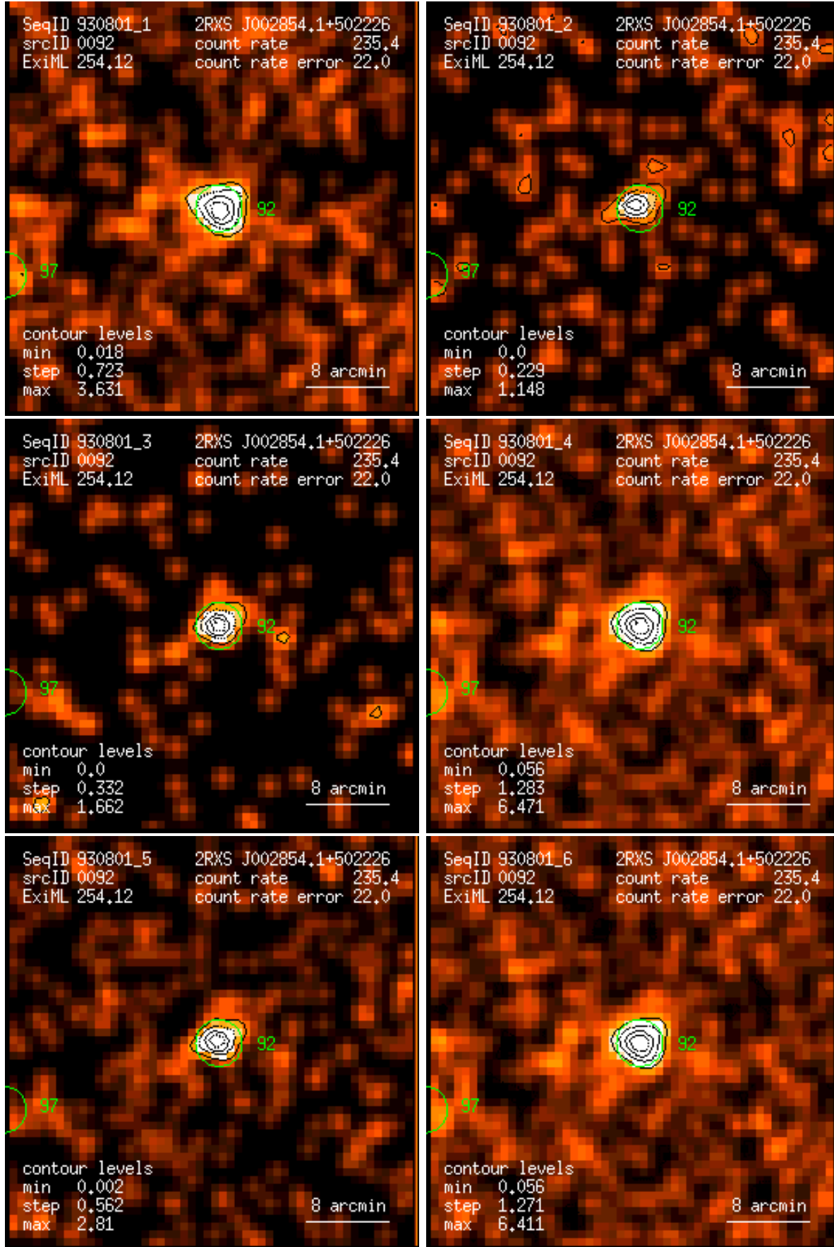
Figure 92: RASS 930801: detection 0092: band rate images, Gaussian filter: (1) PSPC channels 11 – 41, (2) 52 – 90, (3) 91 – 201, (4) 11 – 235, (5) 52 – 201, (6) 11 – 201. Broad band rates in counts/ks. Band rate contour levels in counts/ks/arcmin 2 .
