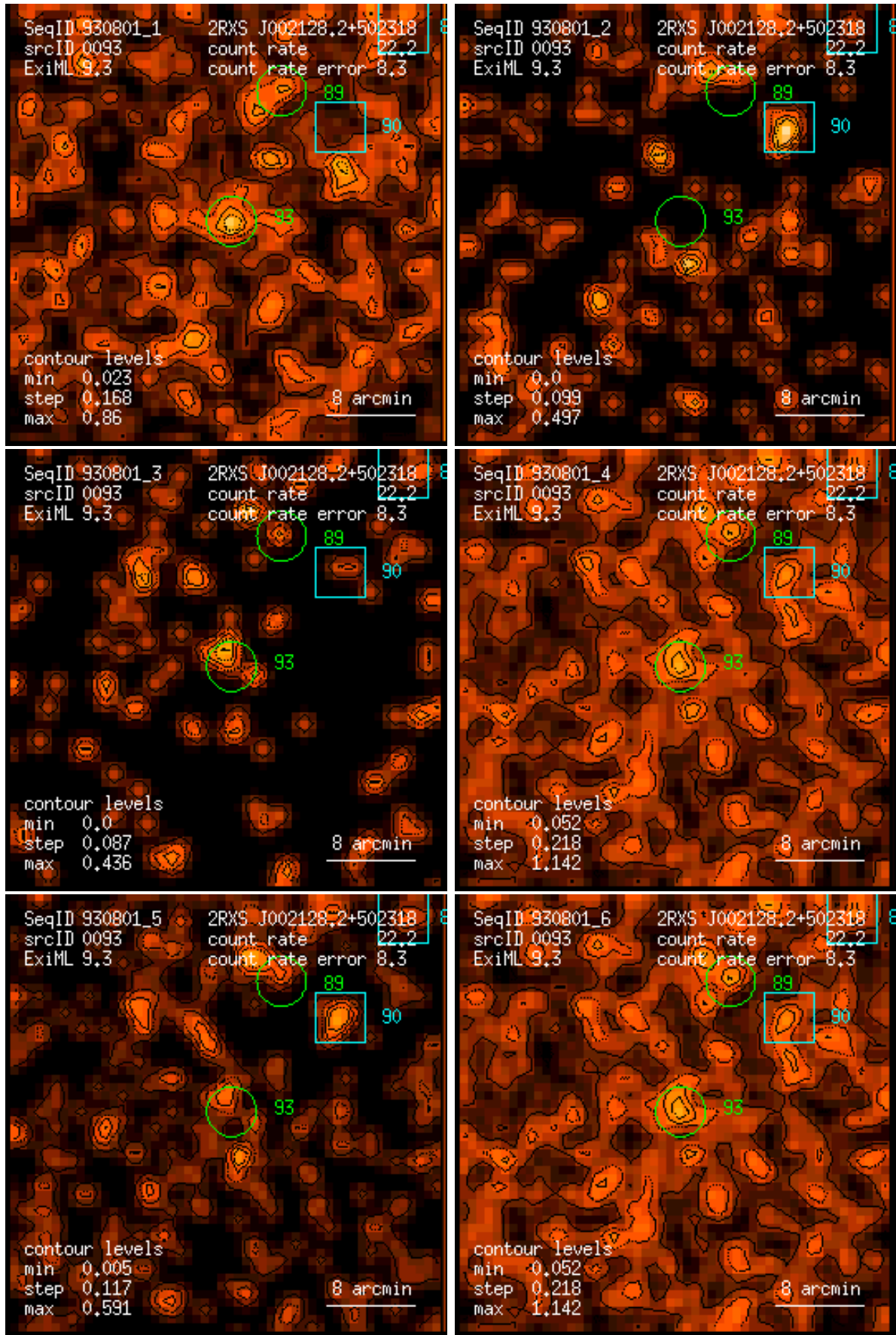
Figure 93: RASS 930801: detection 0093: band rate images, Gaussian filter: (1) PSPC channels 11 – 41, (2) 52 – 90, (3) 91 – 201, (4) 11 – 235, (5) 52 – 201, (6) 11 – 201. Broad band rates in counts/ks. Band rate contour levels in counts/ks/arcmin 2 .
