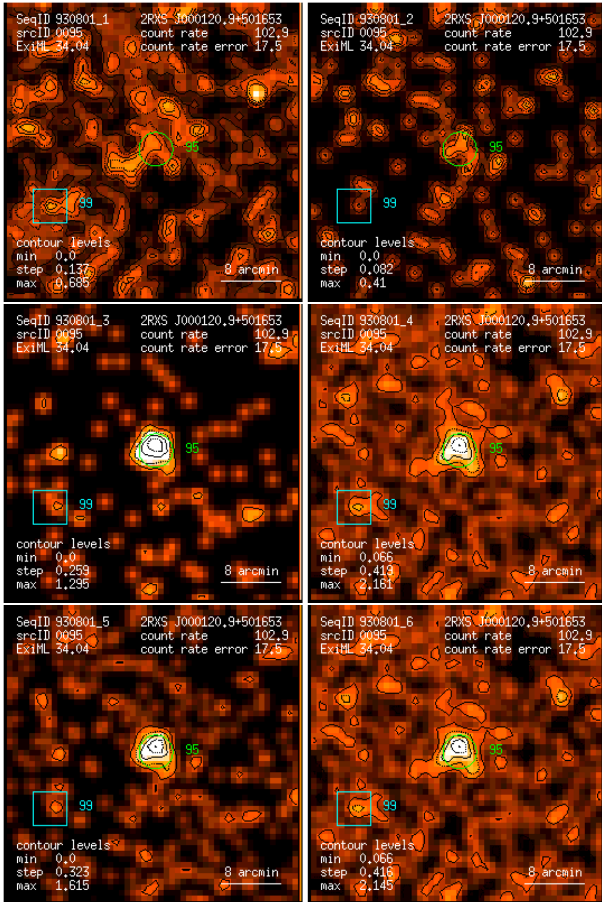
Figure 95: RASS 930801: detection 0095: band rate images, Gaussian filter: (1) PSPC channels 11 – 41, (2) 52 – 90, (3) 91 – 201, (4) 11 – 235, (5) 52 – 201, (6) 11 – 201. Broad band rates in counts/ks. Band rate contour levels in counts/ks/arcmin 2 .
