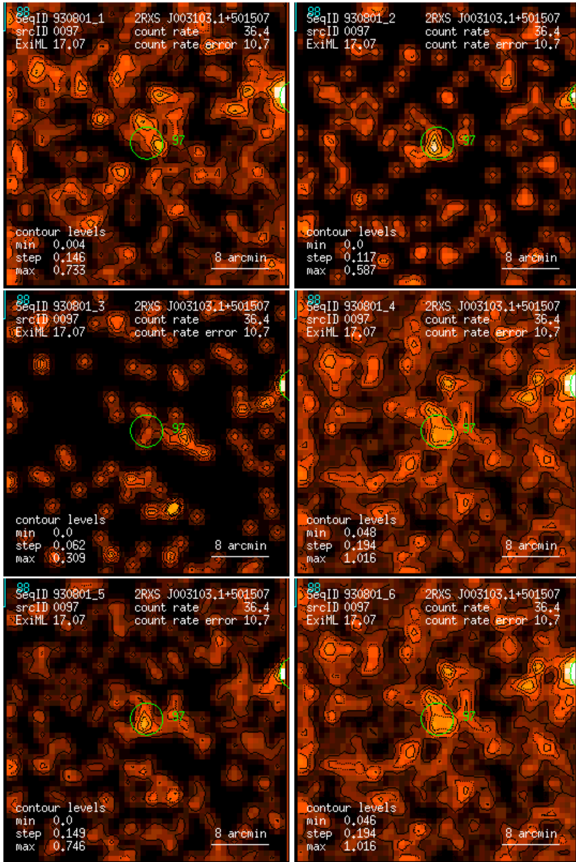
Figure 97: RASS 930801: detection 0097: band rate images, Gaussian filter: (1) PSPC channels 11 – 41, (2) 52 – 90, (3) 91 – 201, (4) 11 – 235, (5) 52 – 201, (6) 11 – 201. Broad band rates in counts/ks. Band rate contour levels in counts/ks/arcmin 2 .
