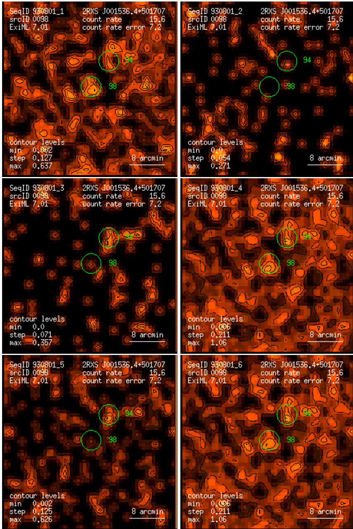
Figure 98: RASS 930801: detection 0098: band rate images, Gaussian filter: (1) PSPC channels 11 – 41, (2) 52 – 90, (3) 91 – 201, (4) 11 – 235, (5) 52 – 201, (6) 11 – 201. Broad band rates in counts/ks. Band rate contour levels in counts/ks/arcmin 2 .
