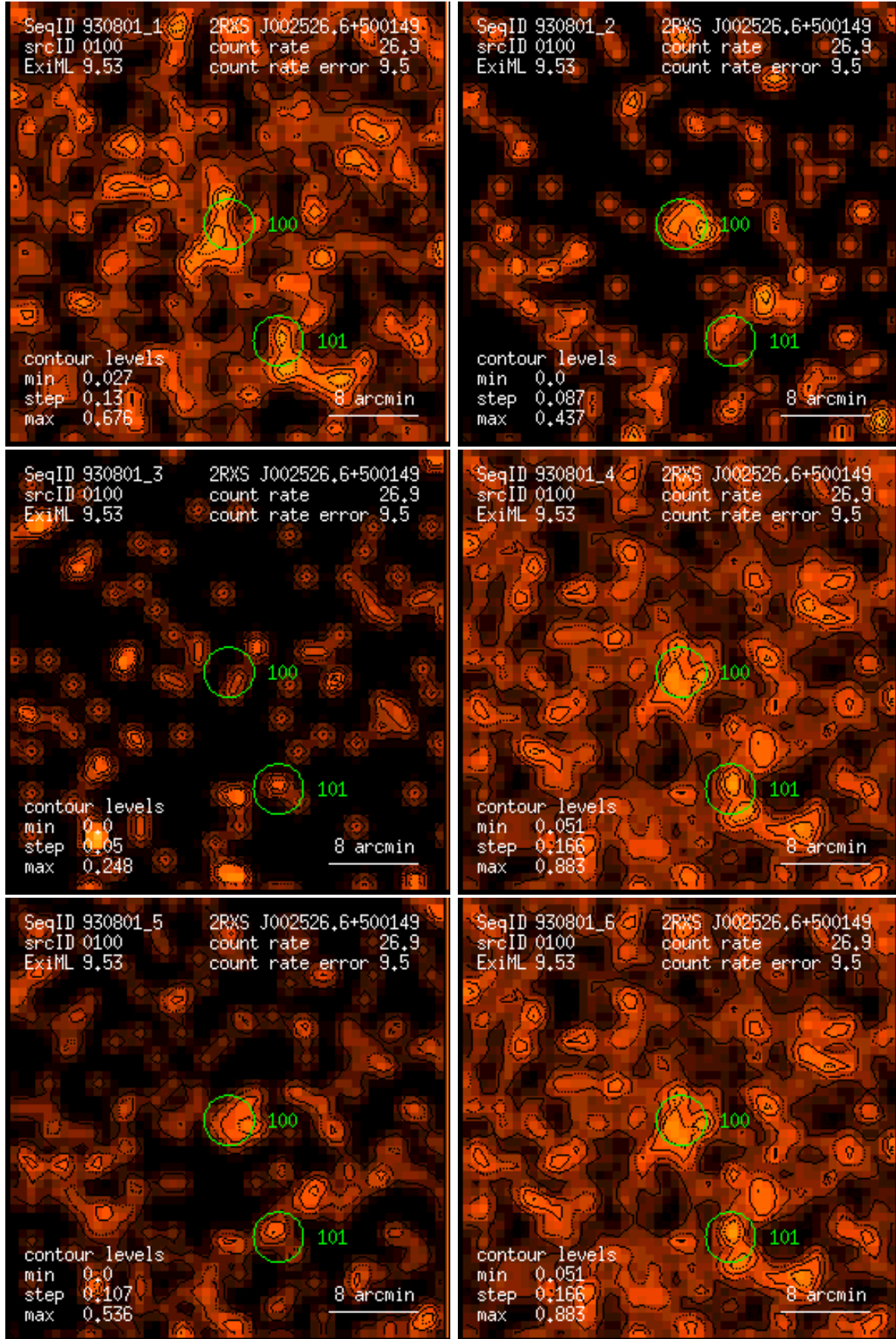
Figure 100: RASS 930801: detection 0100: band rate images, Gaussian filter: (1) PSPC channels 11 – 41, (2) 52 – 90, (3) 91 – 201, (4) 11 – 235, (5) 52 – 201, (6) 11 – 201. Broad band rates in counts/ks. Band rate contour levels in counts/ks/arcmin 2 .
