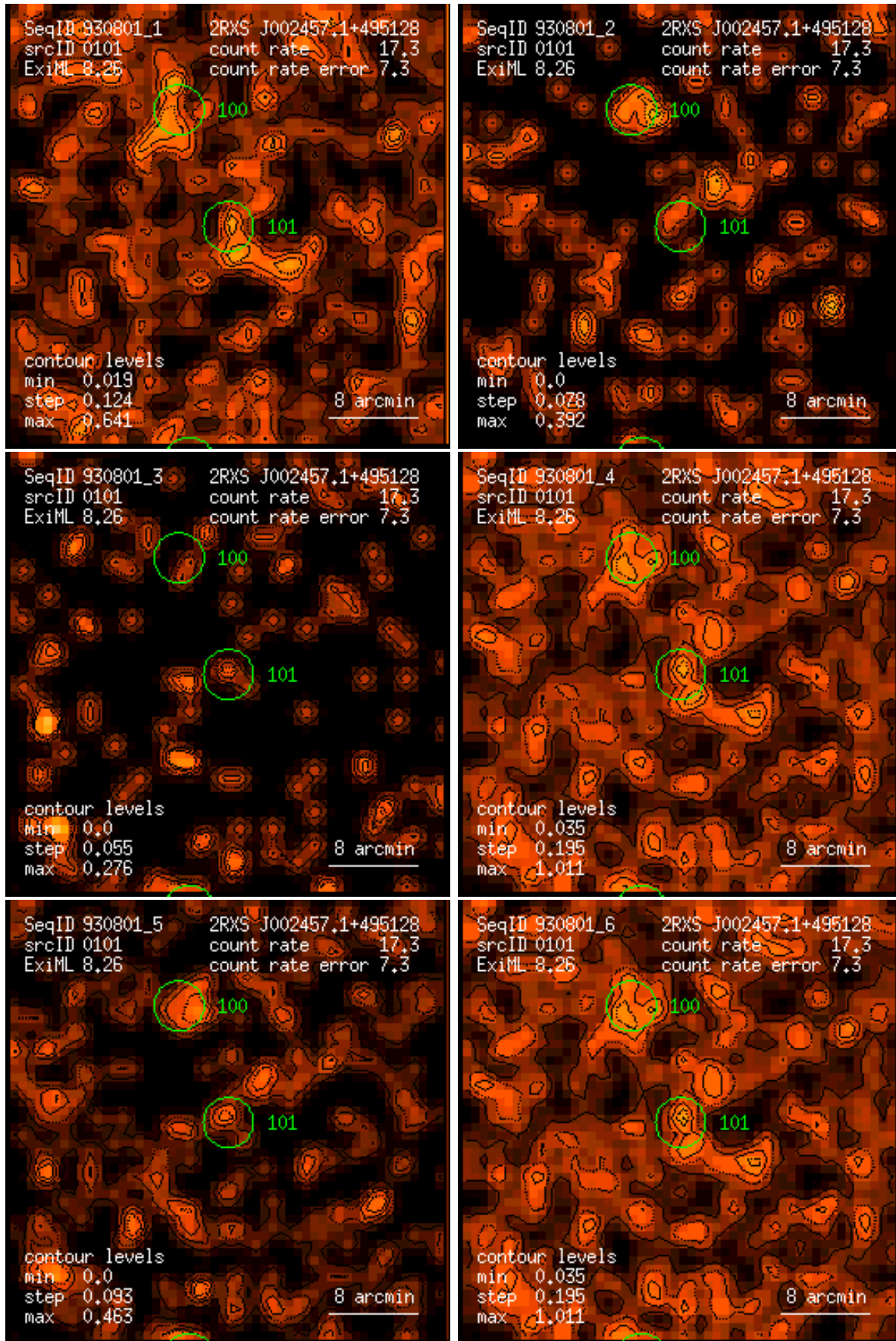
Figure 101: RASS 930801: detection 0101: band rate images, Gaussian filter: (1) PSPC channels 11 – 41, (2) 52 – 90, (3) 91 – 201, (4) 11 – 235, (5) 52 – 201, (6) 11 – 201. Broad band rates in counts/ks. Band rate contour levels in counts/ks/arcmin 2 .
