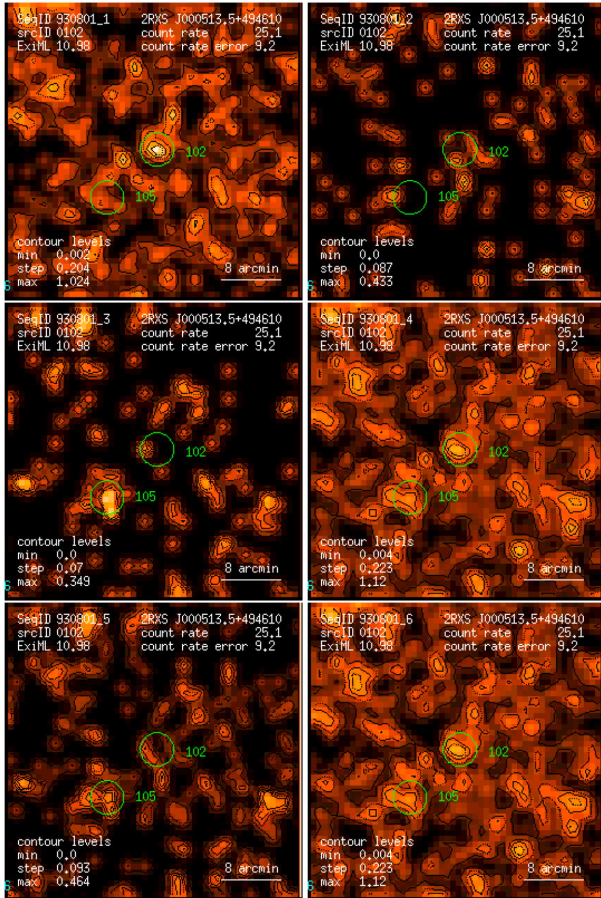
Figure 102: RASS 930801: detection 0102: band rate images, Gaussian filter: (1) PSPC channels 11 – 41, (2) 52 – 90, (3) 91 – 201, (4) 11 – 235, (5) 52 – 201, (6) 11 – 201. Broad band rates in counts/ks. Band rate contour levels in counts/ks/arcmin 2 .
