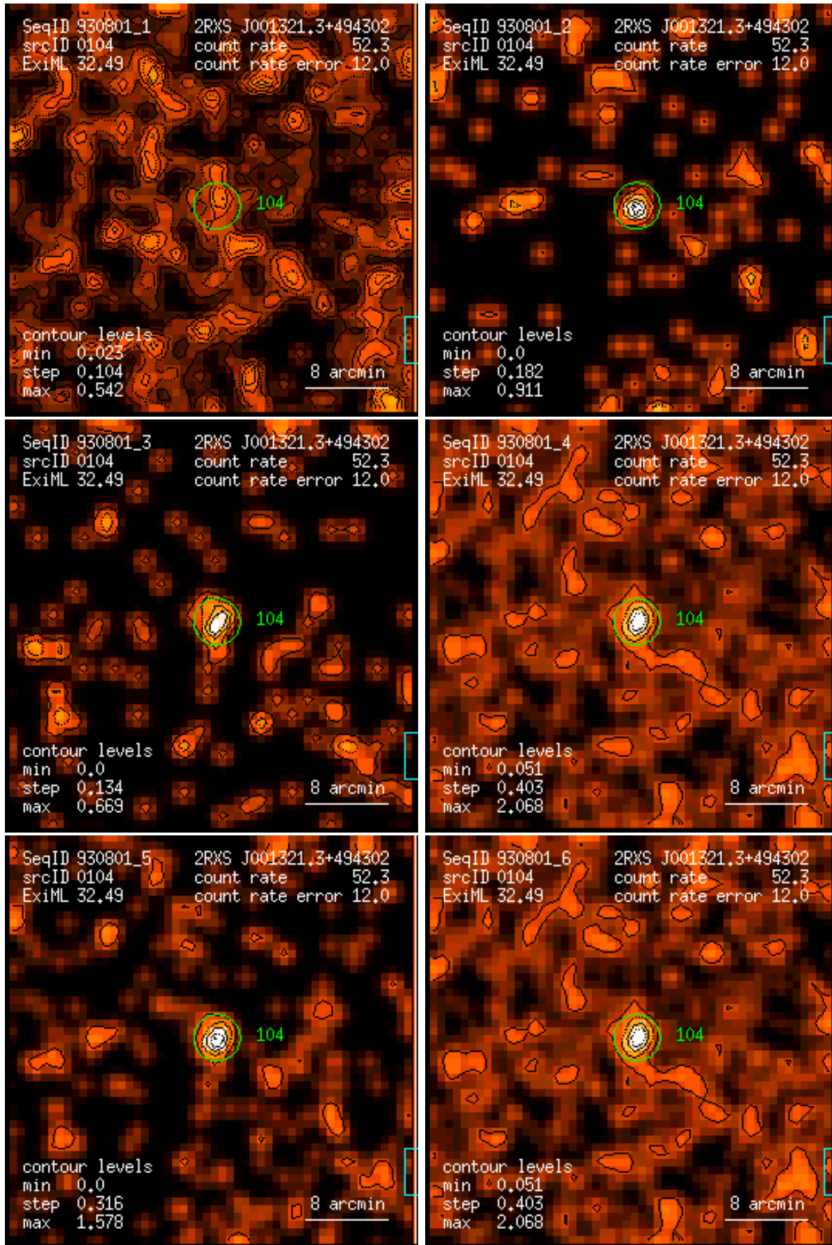
Figure 104: RASS 930801: detection 0104: band rate images, Gaussian filter: (1) PSPC channels 11 – 41, (2) 52 – 90, (3) 91 – 201, (4) 11 – 235, (5) 52 – 201, (6) 11 – 201. Broad band rates in counts/ks. Band rate contour levels in counts/ks/arcmin 2 .
