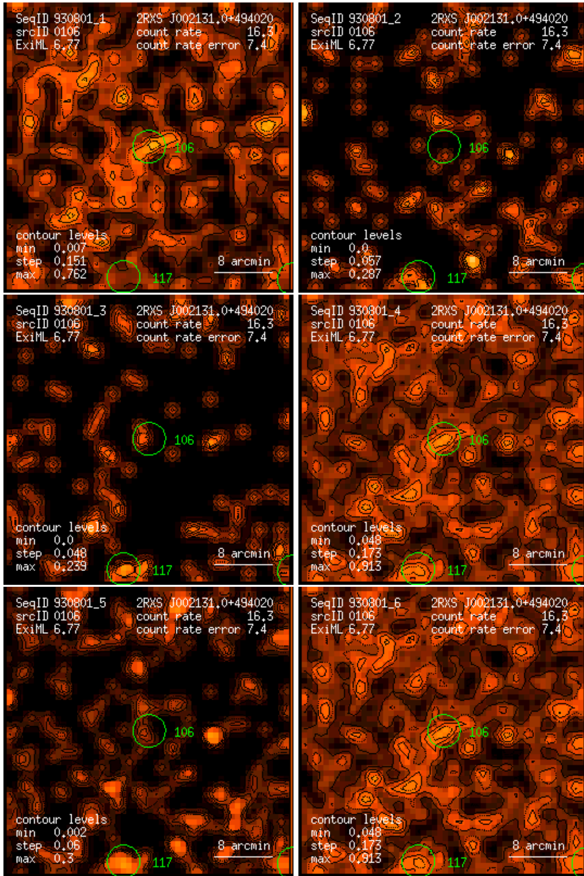
Figure 106: RASS 930801: detection 0106: band rate images, Gaussian filter: (1) PSPC channels 11 – 41, (2) 52 – 90, (3) 91 – 201, (4) 11 – 235, (5) 52 – 201, (6) 11 – 201. Broad band rates in counts/ks. Band rate contour levels in counts/ks/arcmin 2 .
